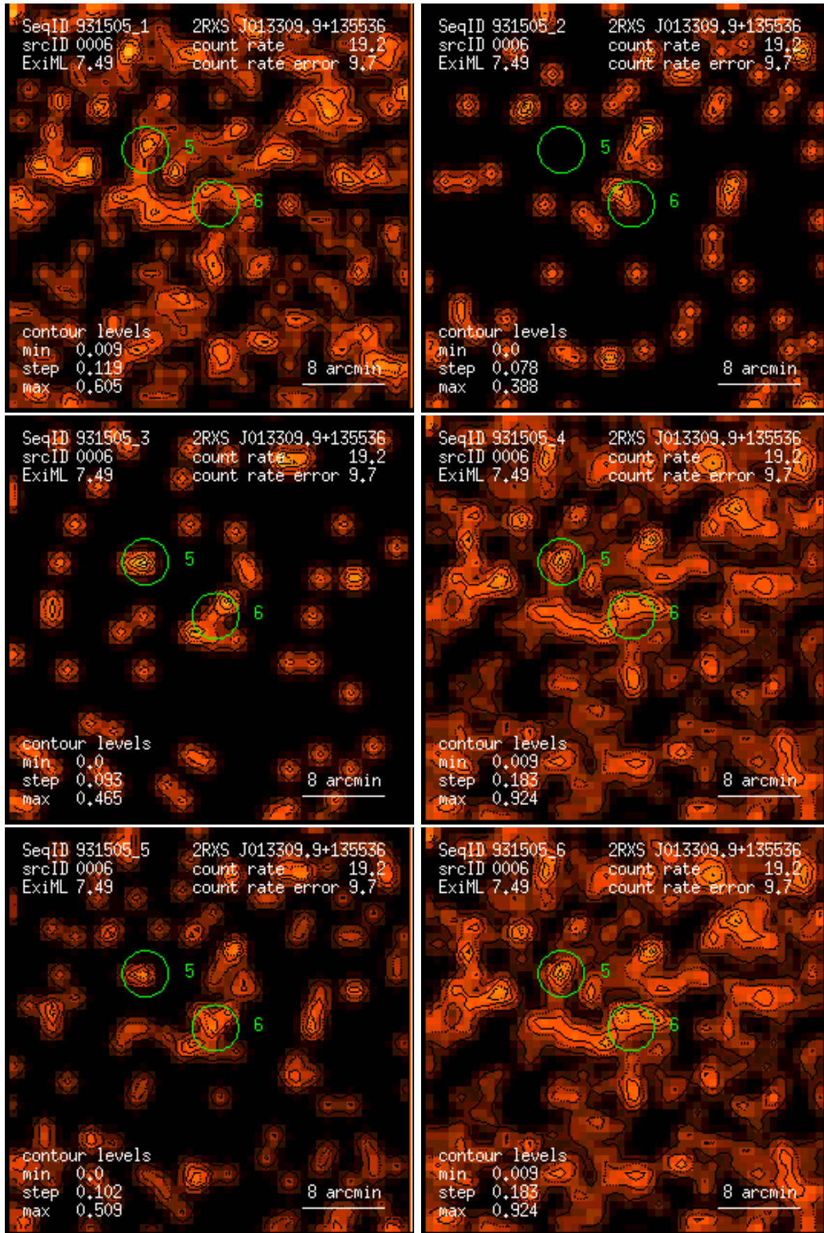
Figure 6: RASS 931505: detection 0006: band rate images, Gaussian filter: (1) PSPC channels 11 – 41, (2) 52 – 90, (3) 91 – 201, (4) 11 – 235, (5) 52 – 201, (6) 11 – 201. Broad band rates in counts/ks. Band rate contour levels in counts/ks/arcmin 2 .
