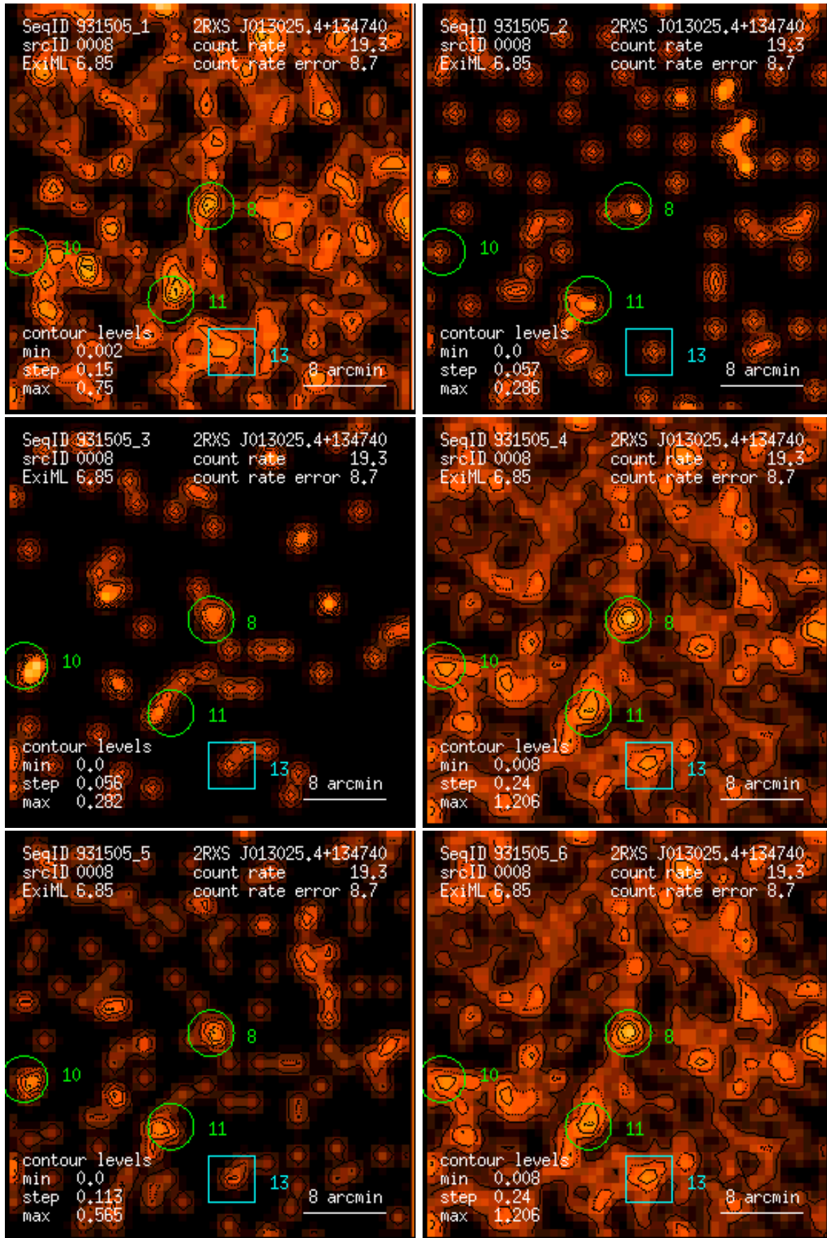
Figure 8: RASS 931505: detection 0008: band rate images, Gaussian filter: (1) PSPC channels 11 – 41, (2) 52 – 90, (3) 91 – 201, (4) 11 – 235, (5) 52 – 201, (6) 11 – 201. Broad band rates in counts/ks. Band rate contour levels in counts/ks/arcmin 2 .
