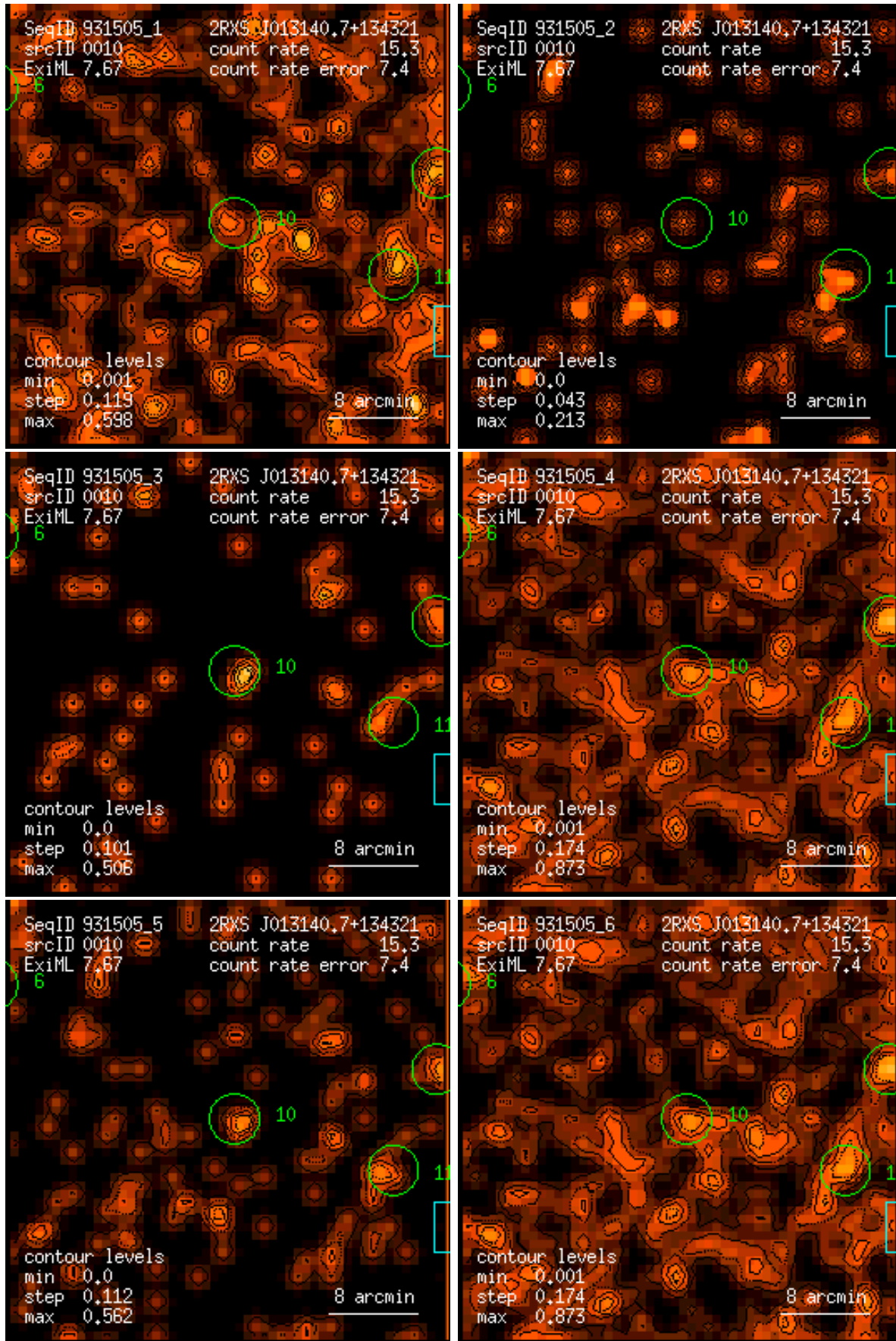
Figure 10: RASS 931505: detection 0010: band rate images, Gaussian filter: (1) PSPC channels 11 – 41, (2) 52 – 90, (3) 91 – 201, (4) 11 – 235, (5) 52 – 201, (6) 11 – 201. Broad band rates in counts/ks. Band rate contour levels in counts/ks/arcmin 2 .
