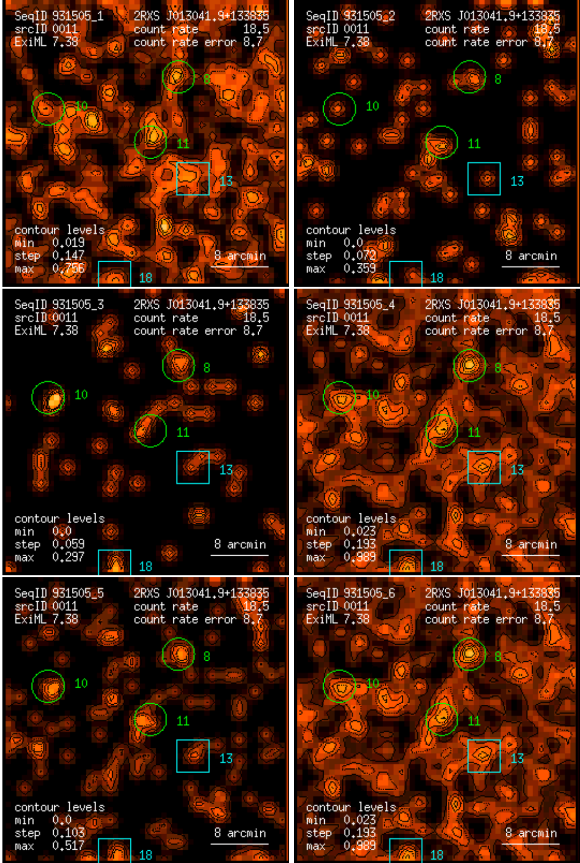
Figure 11: RASS 931505: detection 0011: band rate images, Gaussian filter: (1) PSPC channels 11 – 41, (2) 52 – 90, (3) 91 – 201, (4) 11 – 235, (5) 52 – 201, (6) 11 – 201. Broad band rates in counts/ks. Band rate contour levels in counts/ks/arcmin 2 .
