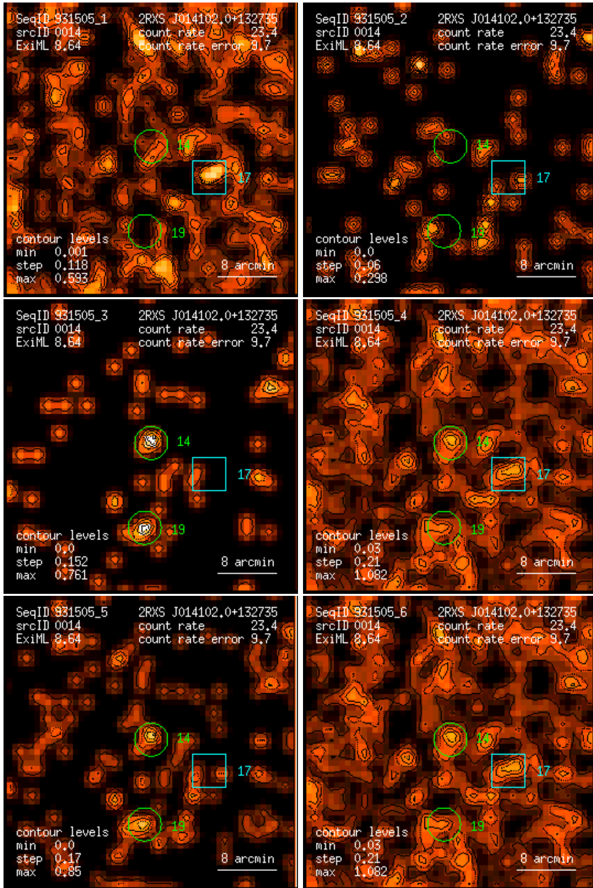
Figure 14: RASS 931505: detection 0014: band rate images, Gaussian filter: (1) PSPC channels 11 – 41, (2) 52 – 90, (3) 91 – 201, (4) 11 – 235, (5) 52 – 201, (6) 11 – 201. Broad band rates in counts/ks. Band rate contour levels in counts/ks/arcmin 2 .
