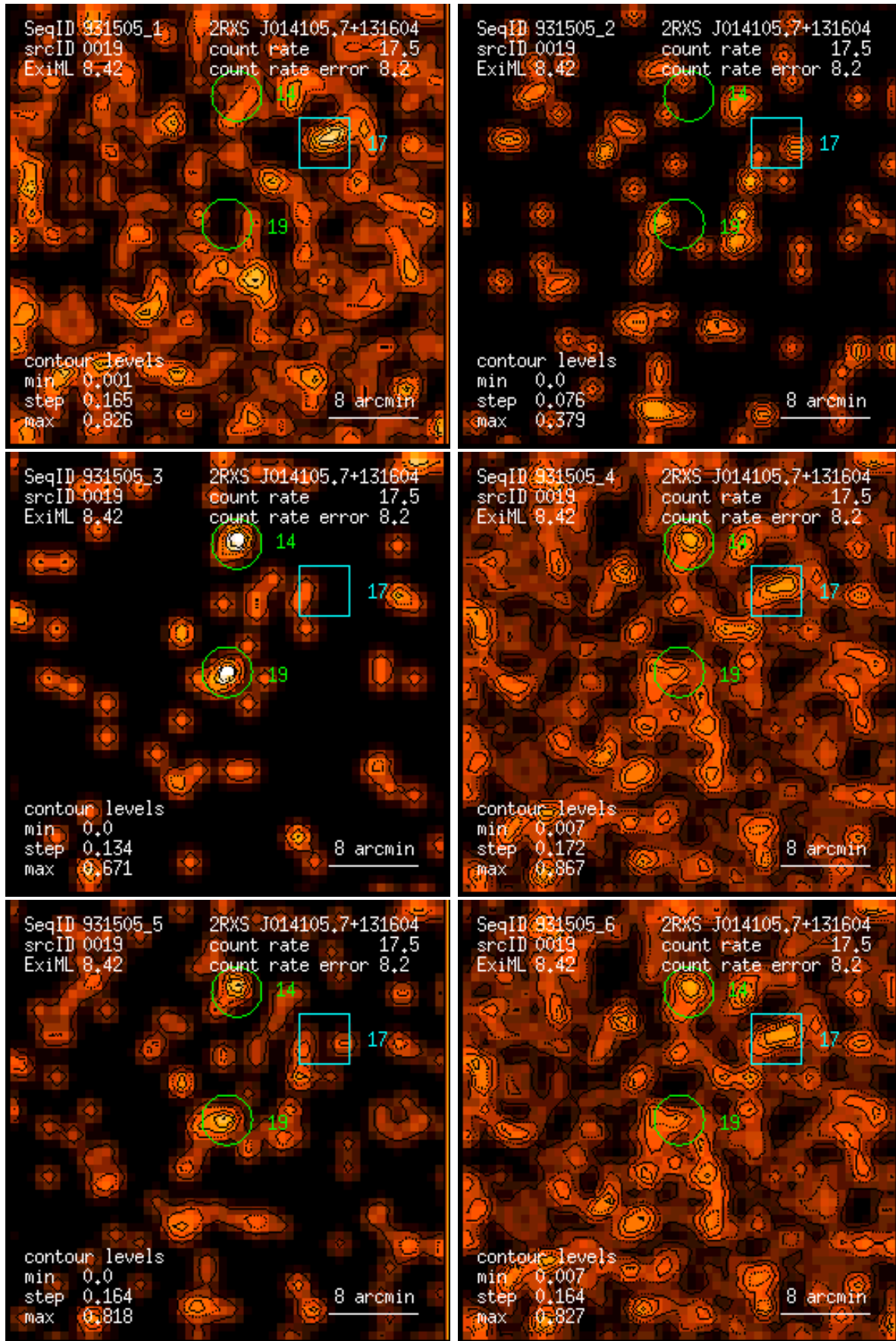
Figure 19: RASS 931505: detection 0019: band rate images, Gaussian filter: (1) PSPC channels 11 – 41, (2) 52 – 90, (3) 91 – 201, (4) 11 – 235, (5) 52 – 201, (6) 11 – 201. Broad band rates in counts/ks. Band rate contour levels in counts/ks/arcmin 2 .
