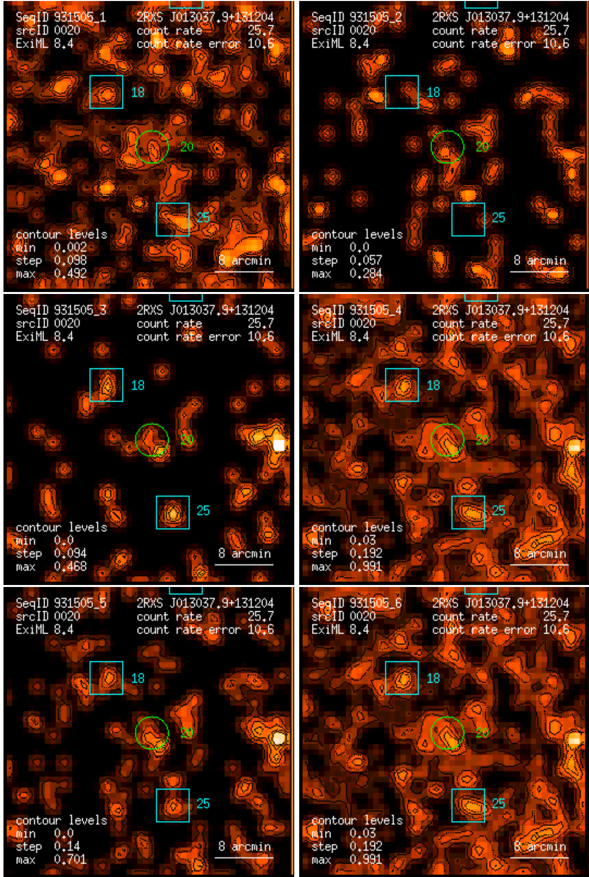
Figure 20: RASS 931505: detection 0020: band rate images, Gaussian filter: (1) PSPC channels 11 – 41, (2) 52 – 90, (3) 91 – 201, (4) 11 – 235, (5) 52 – 201, (6) 11 – 201. Broad band rates in counts/ks. Band rate contour levels in counts/ks/arcmin 2 .
