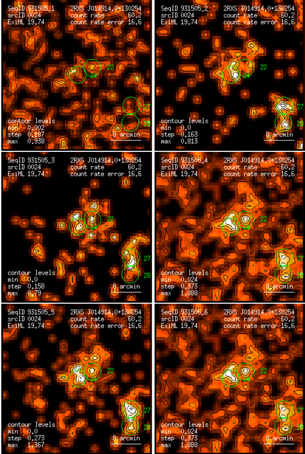
Figure 24: RASS 931505: detection 0024: band rate images, Gaussian filter: (1) PSPC channels 11 – 41, (2) 52 – 90, (3) 91 – 201, (4) 11 – 235, (5) 52 – 201, (6) 11 – 201. Broad band rates in counts/ks. Band rate contour levels in counts/ks/arcmin 2 .
