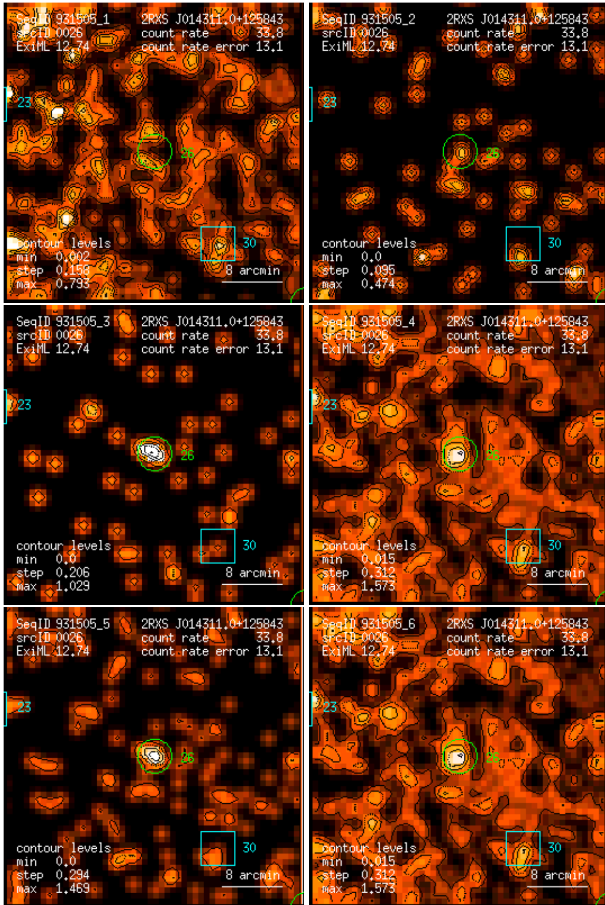
Figure 26: RASS 931505: detection 0026: band rate images, Gaussian filter: (1) PSPC channels 11 – 41, (2) 52 – 90, (3) 91 – 201, (4) 11 – 235, (5) 52 – 201, (6) 11 – 201. Broad band rates in counts/ks. Band rate contour levels in counts/ks/arcmin 2 .
