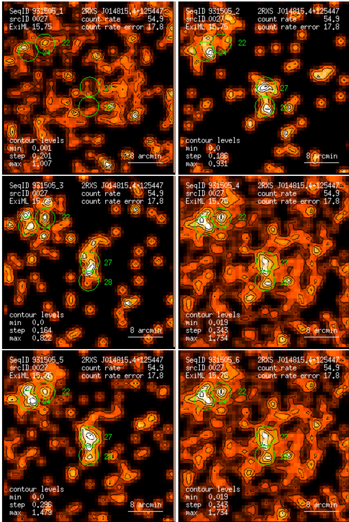
Figure 27: RASS 931505: detection 0027: band rate images, Gaussian filter: (1) PSPC channels 11 – 41, (2) 52 – 90, (3) 91 – 201, (4) 11 – 235, (5) 52 – 201, (6) 11 – 201. Broad band rates in counts/ks. Band rate contour levels in counts/ks/arcmin 2 .
