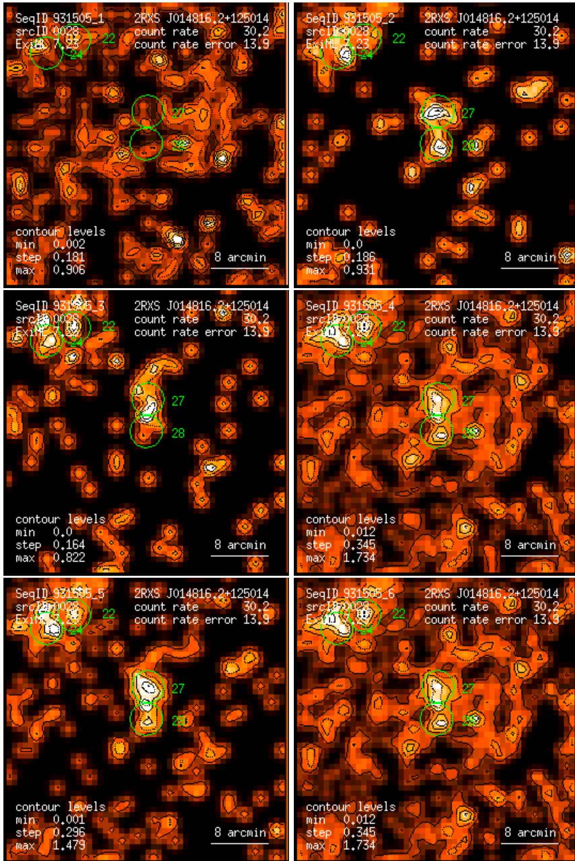
Figure 28: RASS 931505: detection 0028: band rate images, Gaussian filter: (1) PSPC channels 11 – 41, (2) 52 – 90, (3) 91 – 201, (4) 11 – 235, (5) 52 – 201, (6) 11 – 201. Broad band rates in counts/ks. Band rate contour levels in counts/ks/arcmin 2 .
