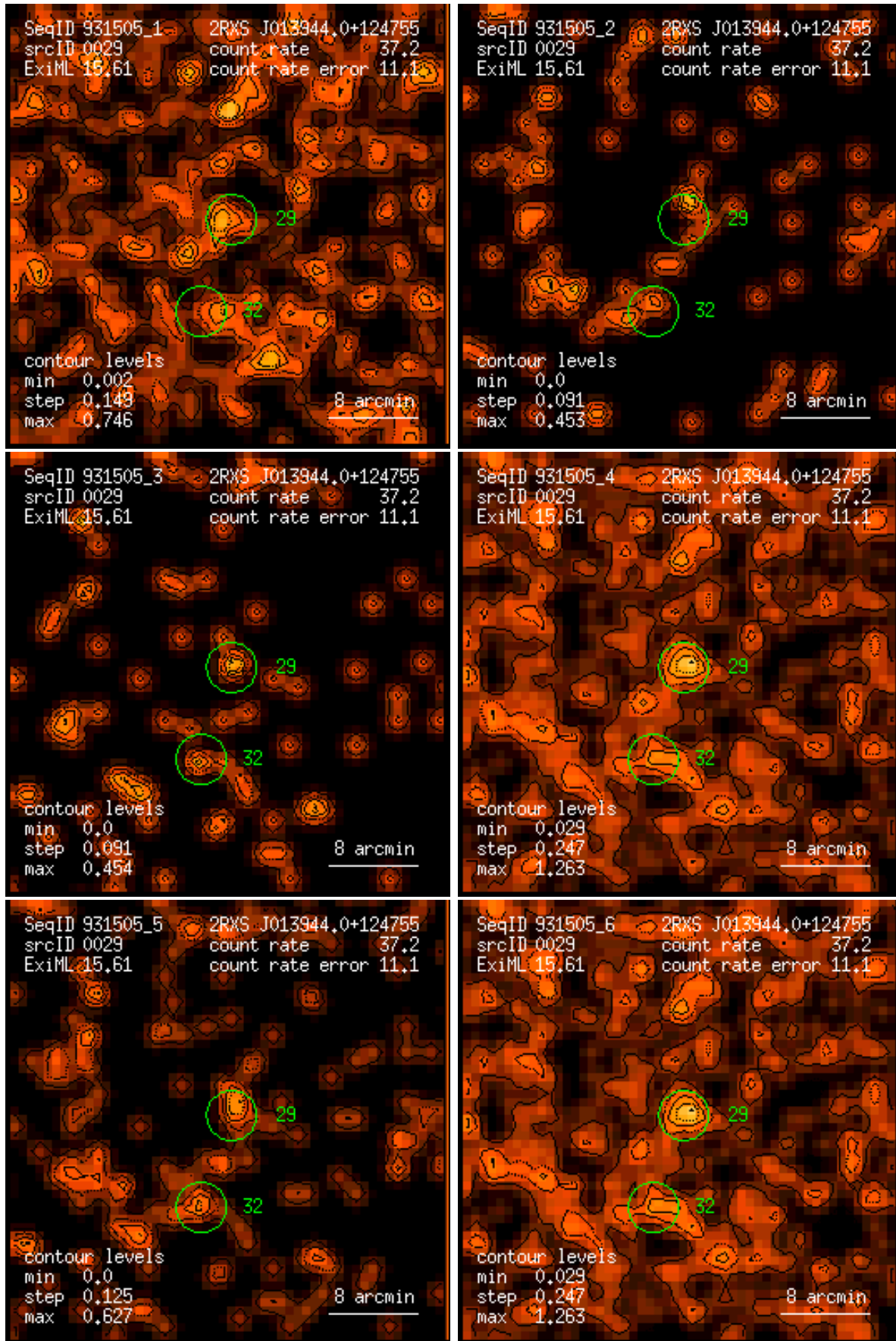
Figure 29: RASS 931505: detection 0029: band rate images, Gaussian filter: (1) PSPC channels 11 – 41, (2) 52 – 90, (3) 91 – 201, (4) 11 – 235, (5) 52 – 201, (6) 11 – 201. Broad band rates in counts/ks. Band rate contour levels in counts/ks/arcmin 2 .
