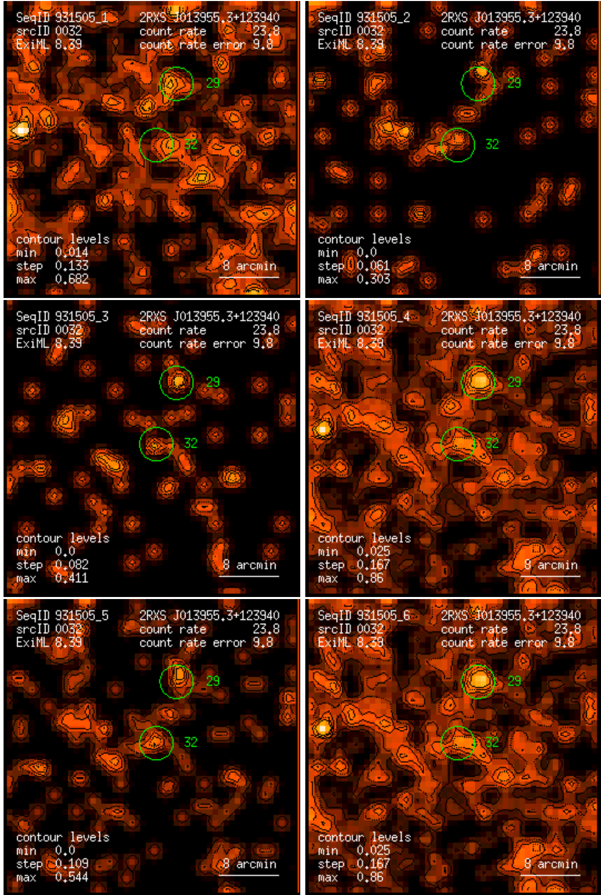
Figure 32: RASS 931505: detection 0032: band rate images, Gaussian filter: (1) PSPC channels 11 – 41, (2) 52 – 90, (3) 91 – 201, (4) 11 – 235, (5) 52 – 201, (6) 11 – 201. Broad band rates in counts/ks. Band rate contour levels in counts/ks/arcmin 2 .
