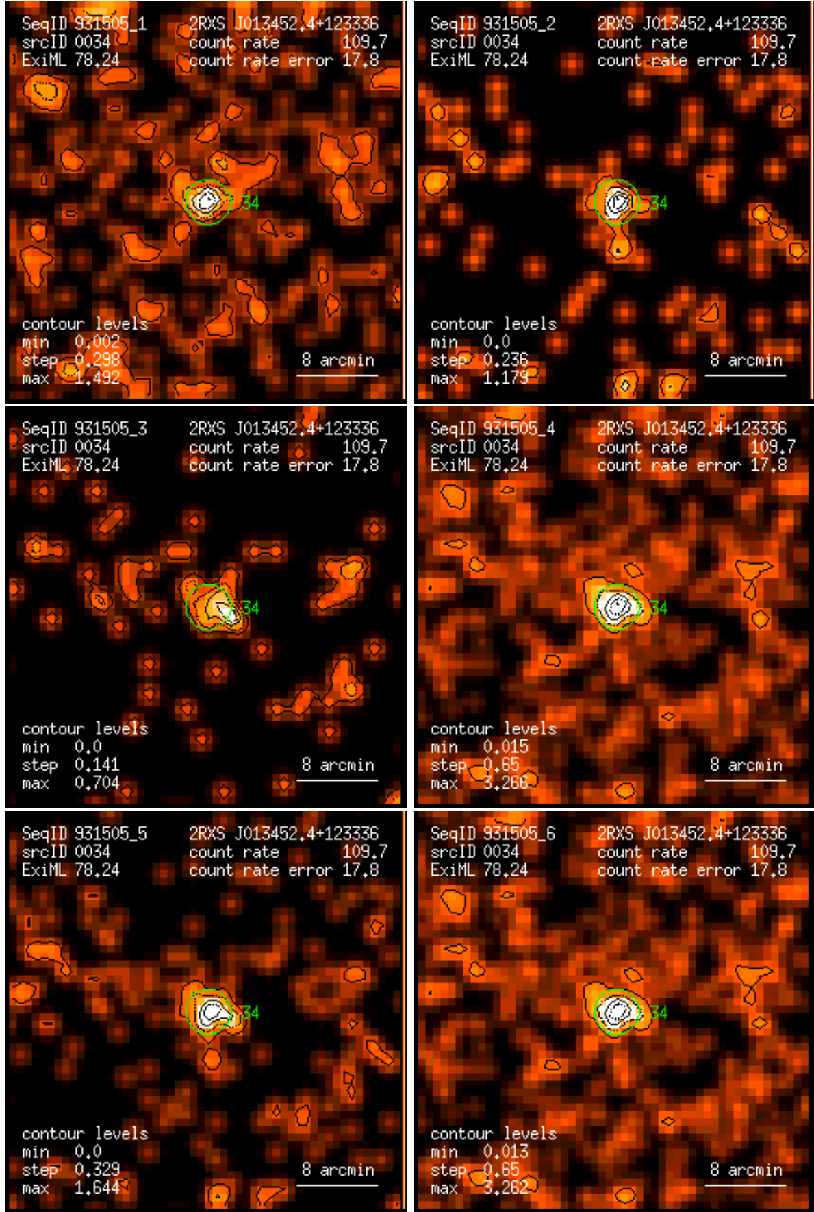
Figure 34: RASS 931505: detection 0034: band rate images, Gaussian filter: (1) PSPC channels 11 – 41, (2) 52 – 90, (3) 91 – 201, (4) 11 – 235, (5) 52 – 201, (6) 11 – 201. Broad band rates in counts/ks. Band rate contour levels in counts/ks/arcmin 2 .
