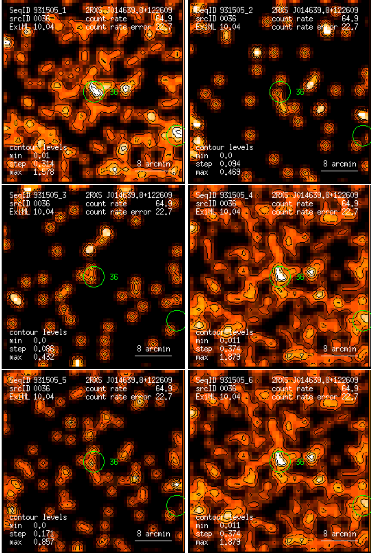
Figure 36: RASS 931505: detection 0036: band rate images, Gaussian filter: (1) PSPC channels 11 – 41, (2) 52 – 90, (3) 91 – 201, (4) 11 – 235, (5) 52 – 201, (6) 11 – 201. Broad band rates in counts/ks. Band rate contour levels in counts/ks/arcmin 2 .
