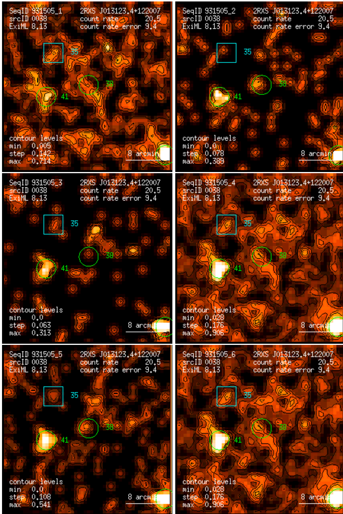
Figure 38: RASS 931505: detection 0038: band rate images, Gaussian filter: (1) PSPC channels 11 – 41, (2) 52 – 90, (3) 91 – 201, (4) 11 – 235, (5) 52 – 201, (6) 11 – 201. Broad band rates in counts/ks. Band rate contour levels in counts/ks/arcmin 2 .
