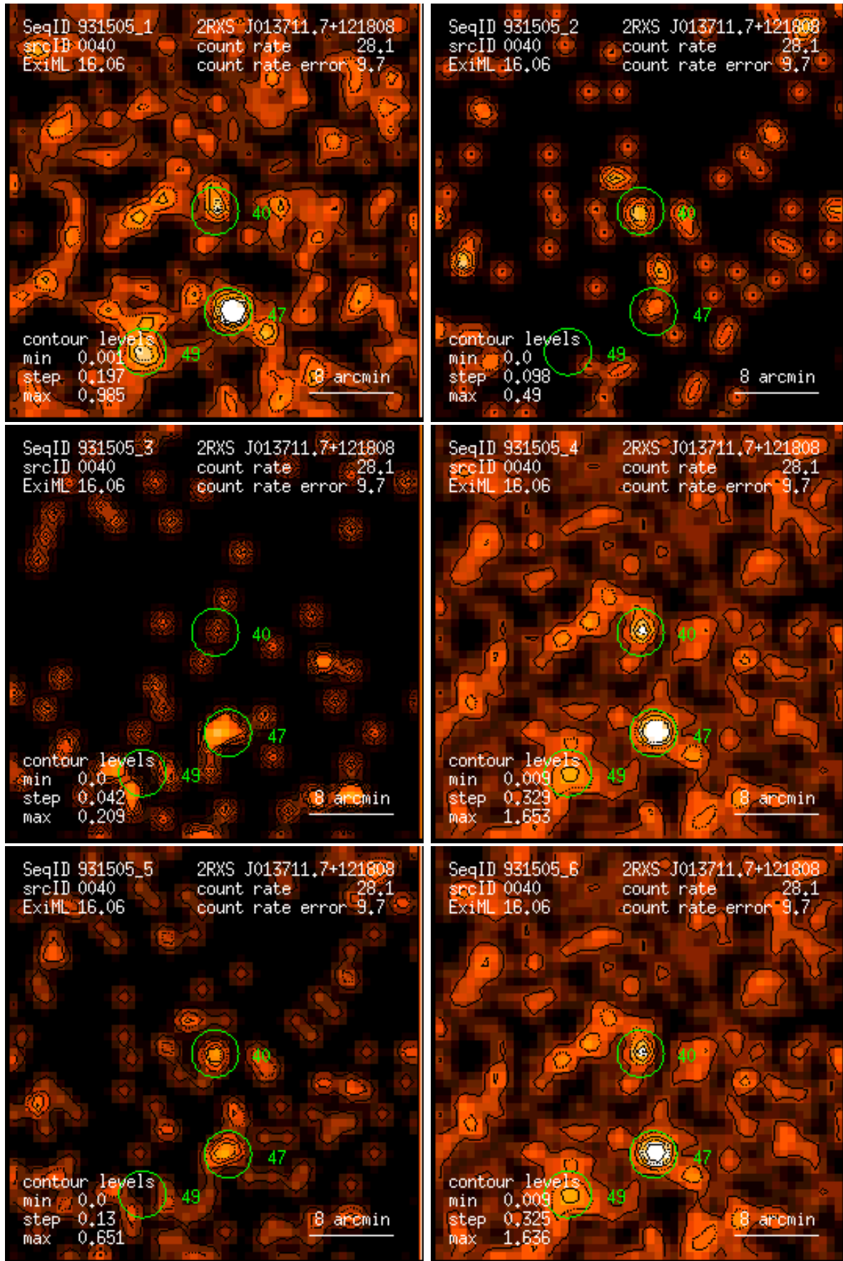
Figure 40: RASS 931505: detection 0040: band rate images, Gaussian filter: (1) PSPC channels 11 – 41, (2) 52 – 90, (3) 91 – 201, (4) 11 – 235, (5) 52 – 201, (6) 11 – 201. Broad band rates in counts/ks. Band rate contour levels in counts/ks/arcmin 2 .
