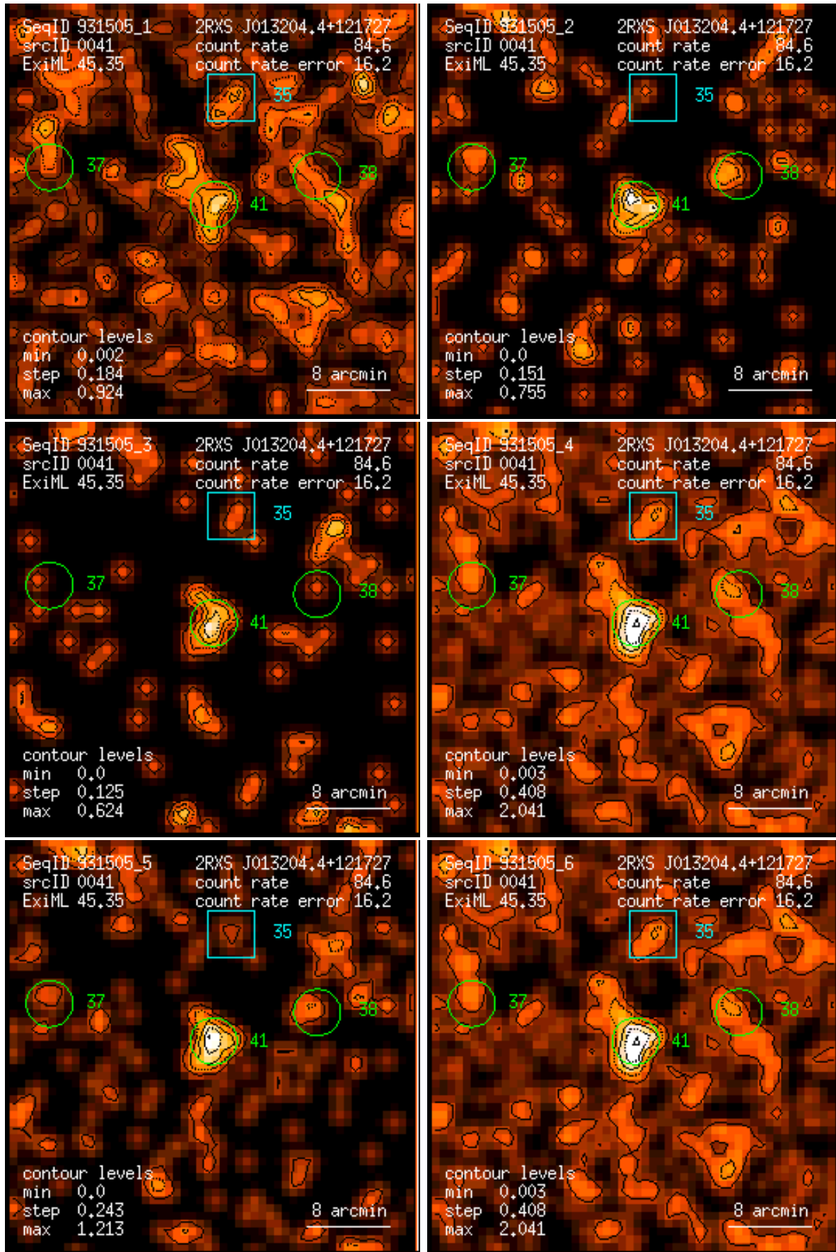
Figure 41: RASS 931505: detection 0041: band rate images, Gaussian filter: (1) PSPC channels 11 – 41, (2) 52 – 90, (3) 91 – 201, (4) 11 – 235, (5) 52 – 201, (6) 11 – 201. Broad band rates in counts/ks. Band rate contour levels in counts/ks/arcmin 2 .
