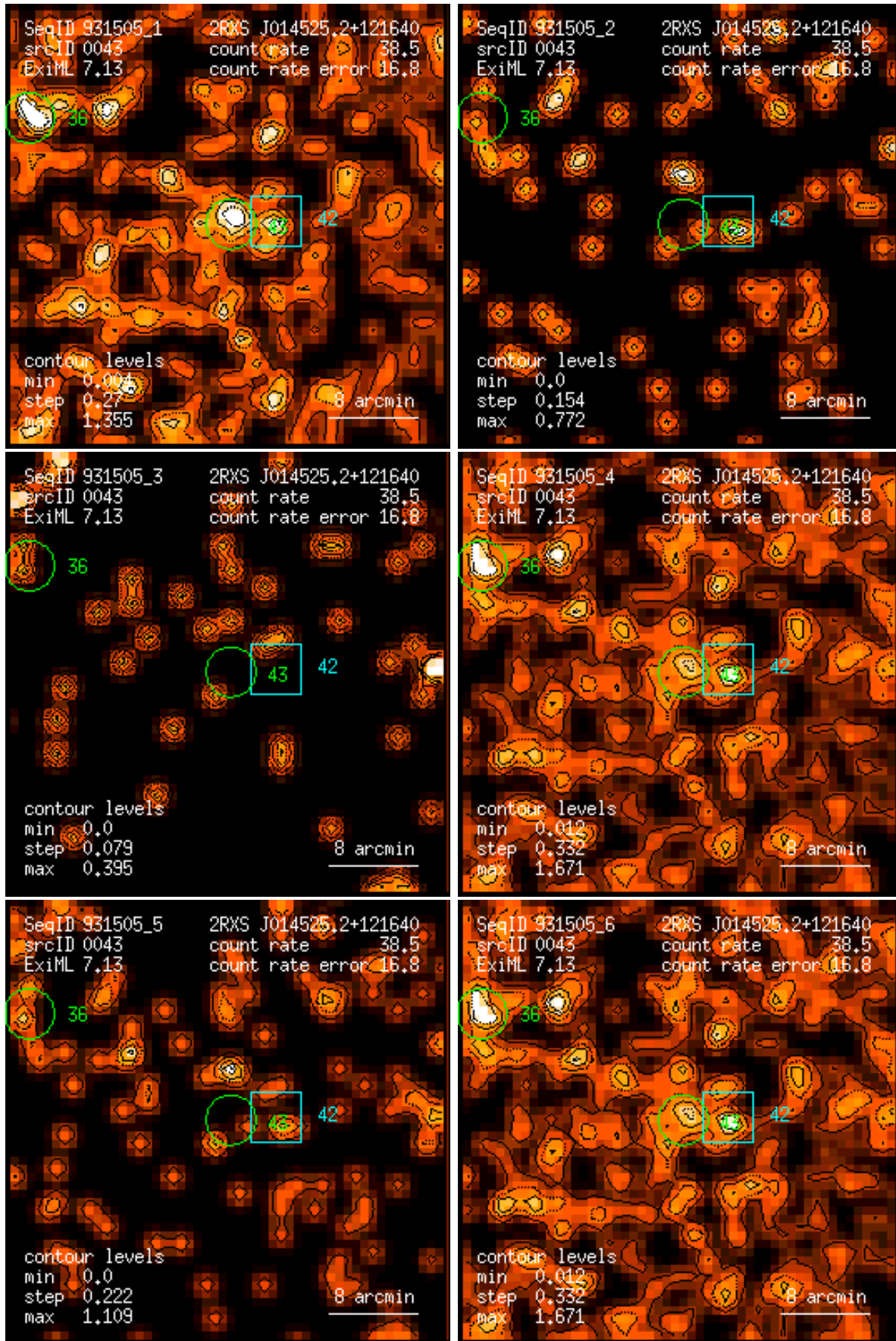
Figure 43: RASS 931505: detection 0043: band rate images, Gaussian filter: (1) PSPC channels 11 – 41, (2) 52 – 90, (3) 91 – 201, (4) 11 – 235, (5) 52 – 201, (6) 11 – 201. Broad band rates in counts/ks. Band rate contour levels in counts/ks/arcmin 2 .
