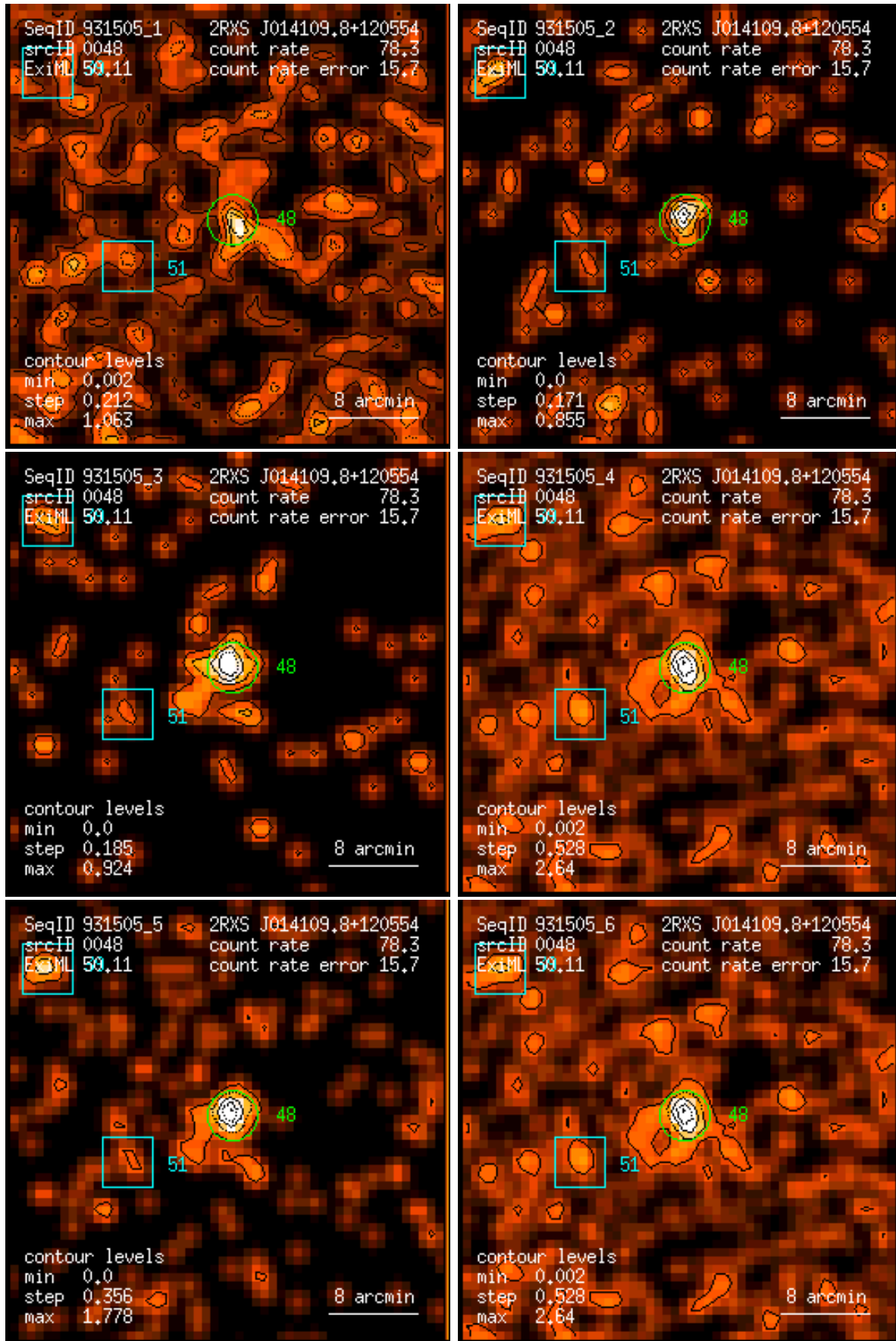
Figure 48: RASS 931505: detection 0048: band rate images, Gaussian filter: (1) PSPC channels 11 – 41, (2) 52 – 90, (3) 91 – 201, (4) 11 – 235, (5) 52 – 201, (6) 11 – 201. Broad band rates in counts/ks. Band rate contour levels in counts/ks/arcmin 2 .
