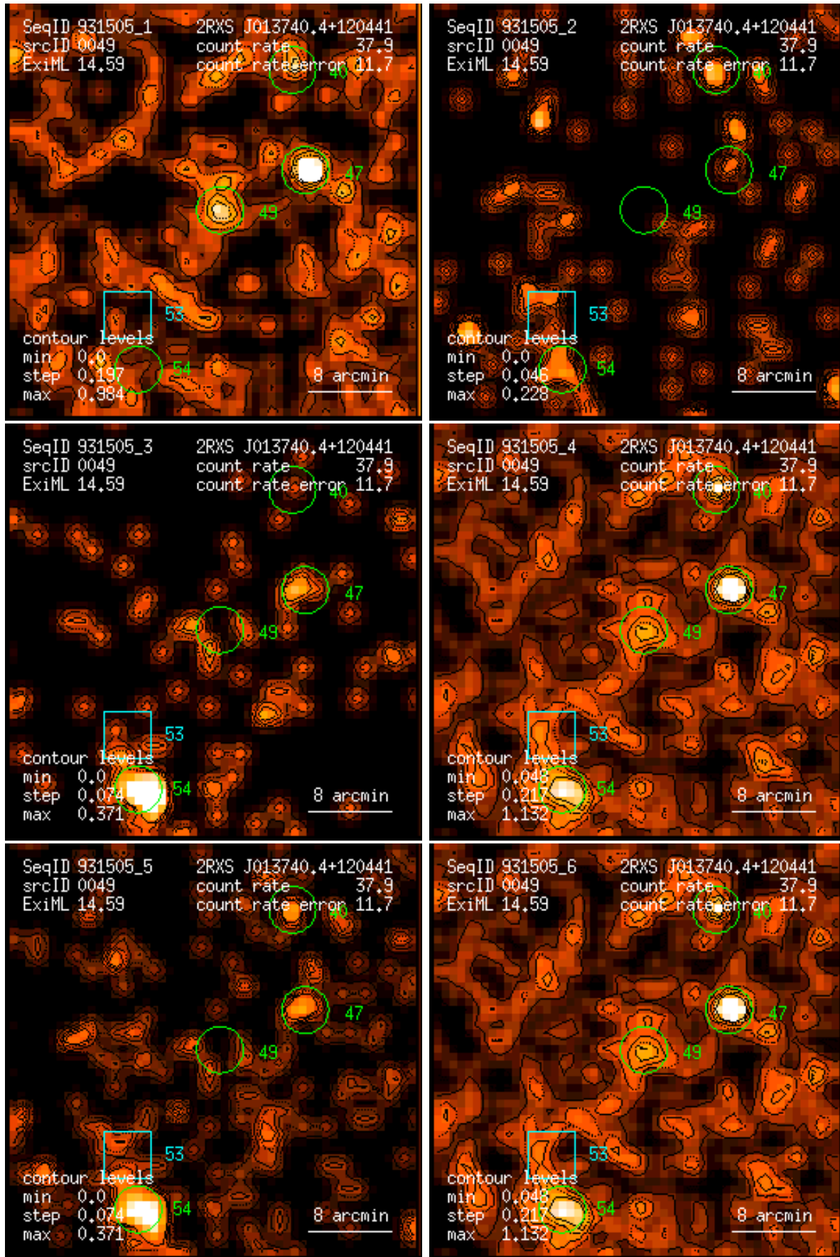
Figure 49: RASS 931505: detection 0049: band rate images, Gaussian filter: (1) PSPC channels 11 – 41, (2) 52 – 90, (3) 91 – 201, (4) 11 – 235, (5) 52 – 201, (6) 11 – 201. Broad band rates in counts/ks. Band rate contour levels in counts/ks/arcmin 2 .
