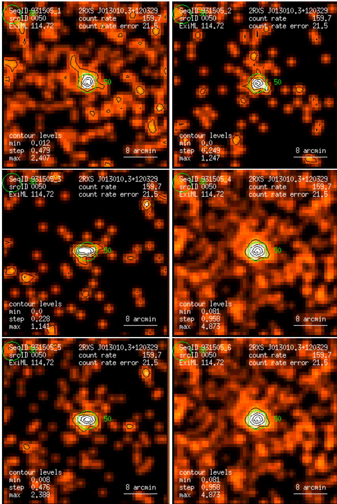
Figure 50: RASS 931505: detection 0050: band rate images, Gaussian filter: (1) PSPC channels 11 – 41, (2) 52 – 90, (3) 91 – 201, (4) 11 – 235, (5) 52 – 201, (6) 11 – 201. Broad band rates in counts/ks. Band rate contour levels in counts/ks/arcmin 2 .
