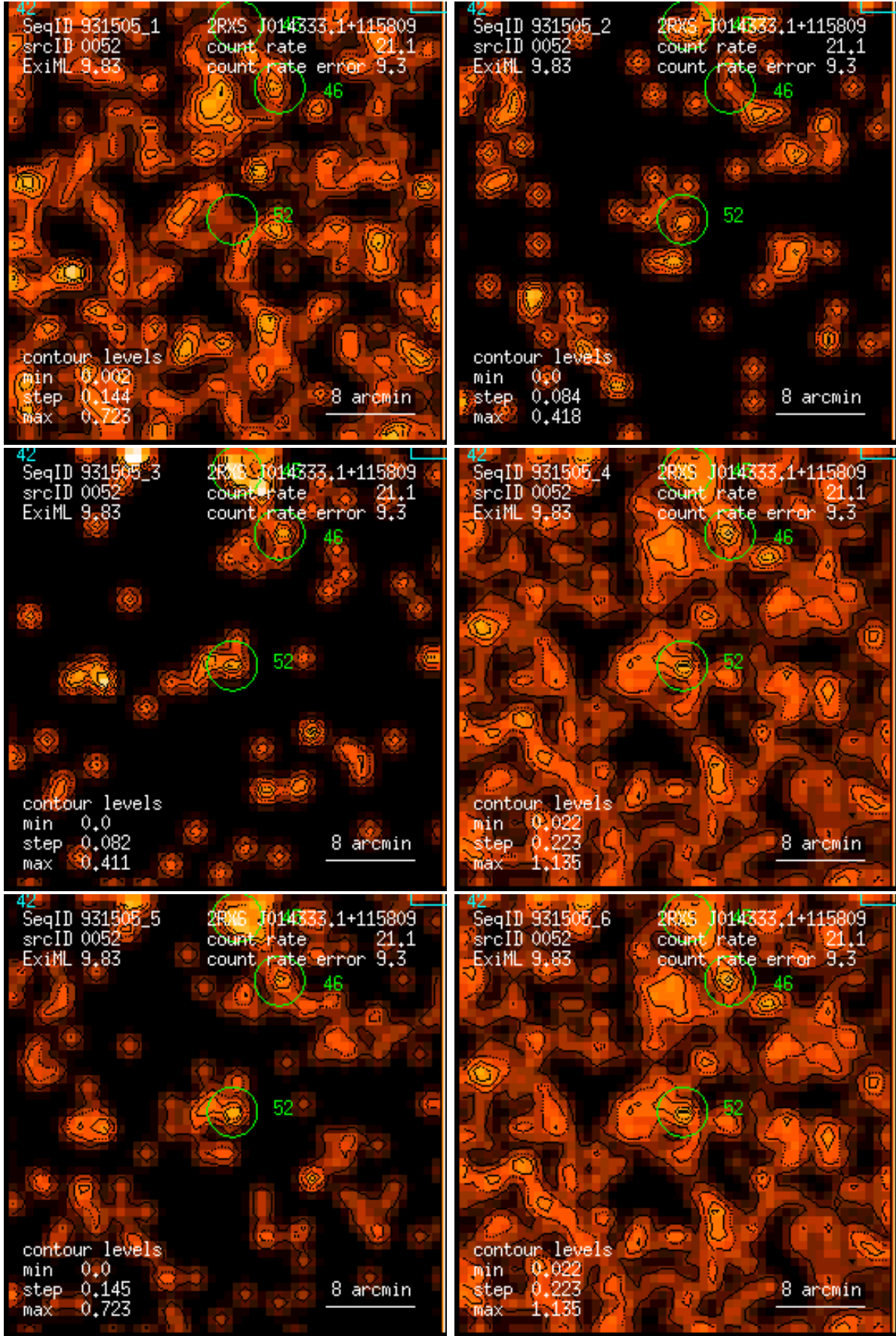
Figure 52: RASS 931505: detection 0052: band rate images, Gaussian filter: (1) PSPC channels 11 – 41, (2) 52 – 90, (3) 91 – 201, (4) 11 – 235, (5) 52 – 201, (6) 11 – 201. Broad band rates in counts/ks. Band rate contour levels in counts/ks/arcmin 2 .
