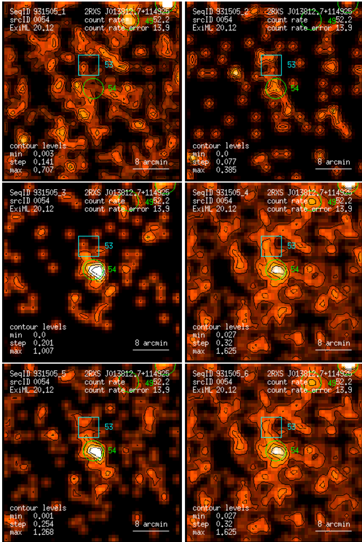
Figure 54: RASS 931505: detection 0054: band rate images, Gaussian filter: (1) PSPC channels 11 – 41, (2) 52 – 90, (3) 91 – 201, (4) 11 – 235, (5) 52 – 201, (6) 11 – 201. Broad band rates in counts/ks. Band rate contour levels in counts/ks/arcmin 2 .
