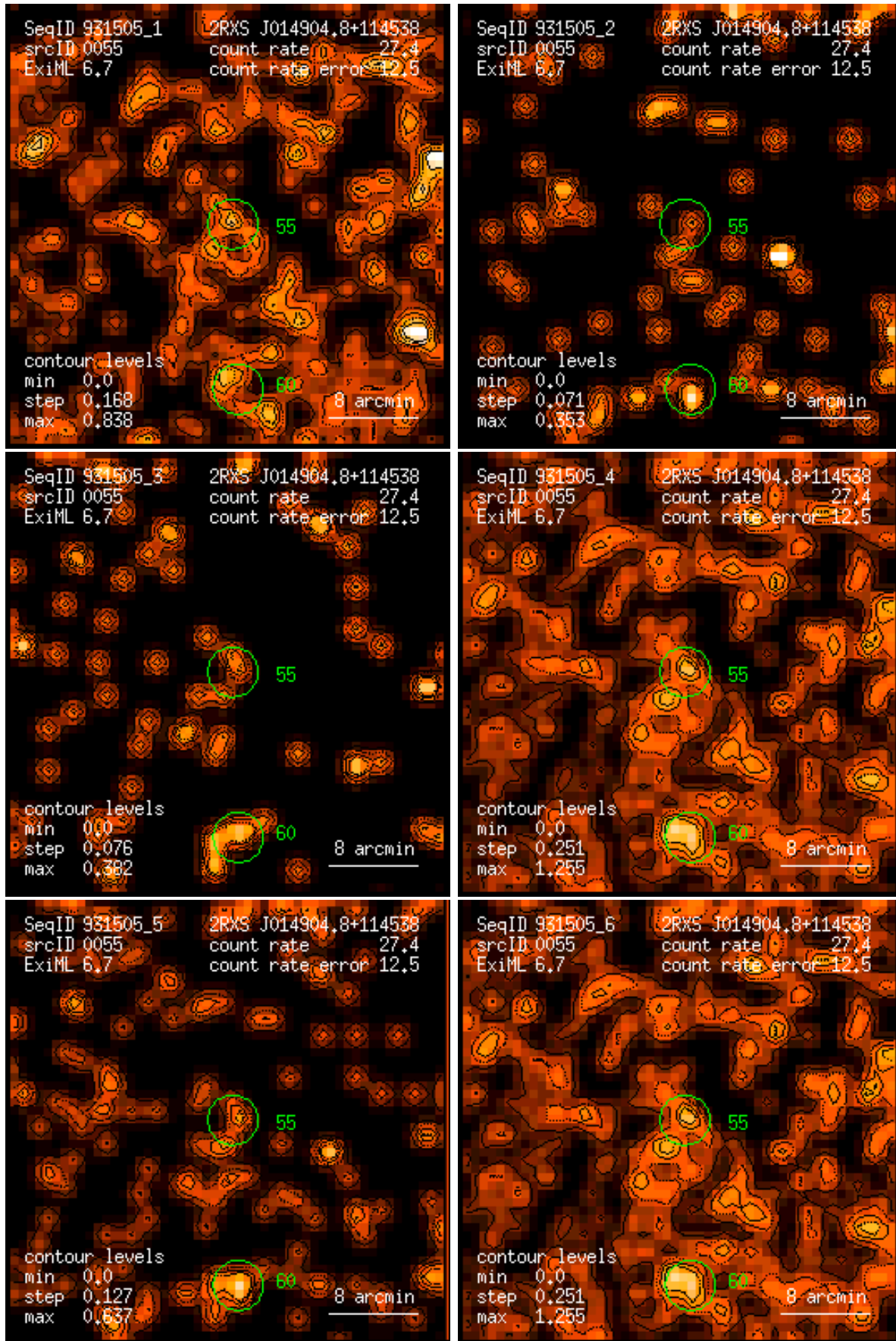
Figure 55: RASS 931505: detection 0055: band rate images, Gaussian filter: (1) PSPC channels 11 – 41, (2) 52 – 90, (3) 91 – 201, (4) 11 – 235, (5) 52 – 201, (6) 11 – 201. Broad band rates in counts/ks. Band rate contour levels in counts/ks/arcmin 2 .
