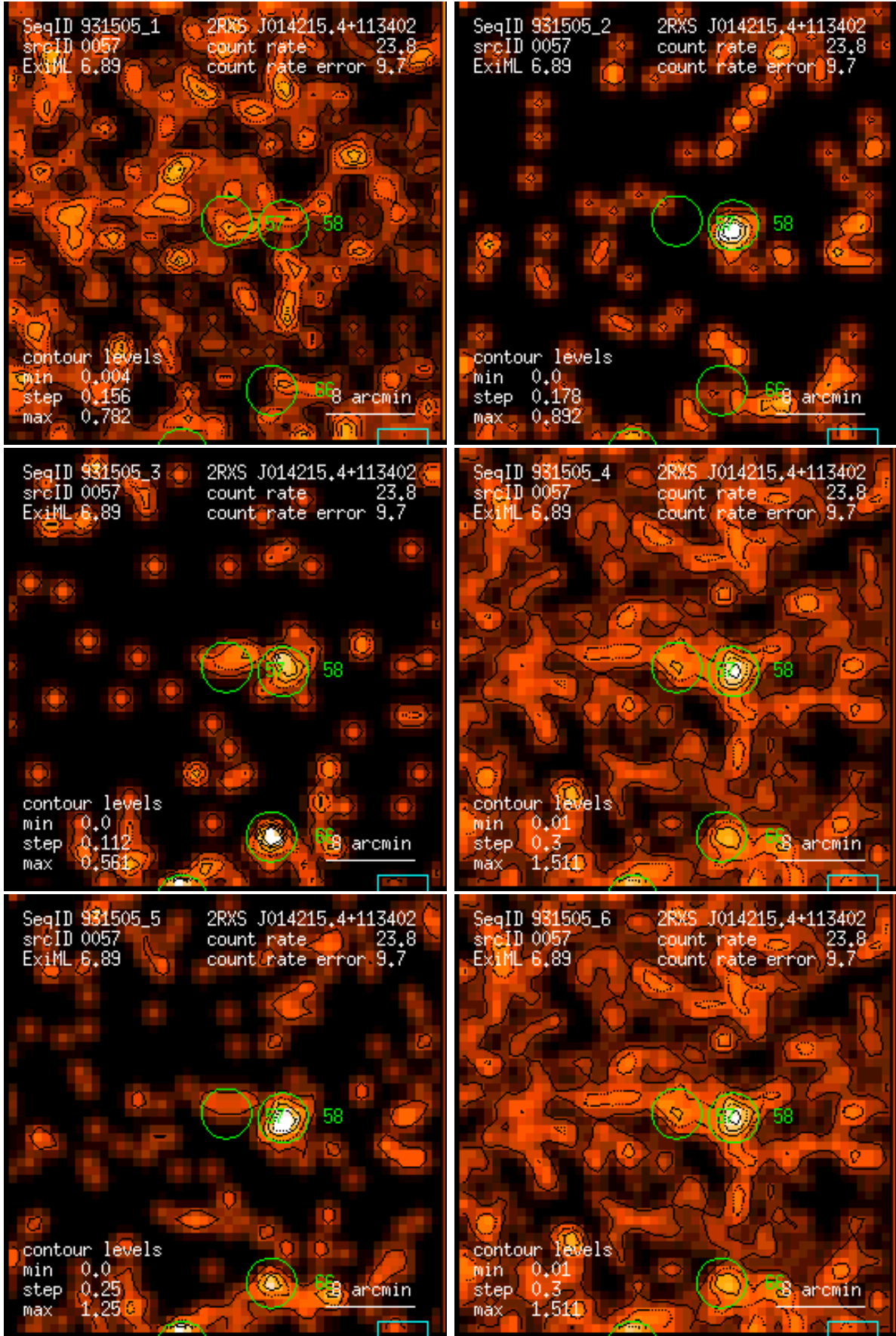
Figure 57: RASS 931505: detection 0057: band rate images, Gaussian filter: (1) PSPC channels 11 – 41, (2) 52 – 90, (3) 91 – 201, (4) 11 – 235, (5) 52 – 201, (6) 11 – 201. Broad band rates in counts/ks. Band rate contour levels in counts/ks/arcmin 2 .
