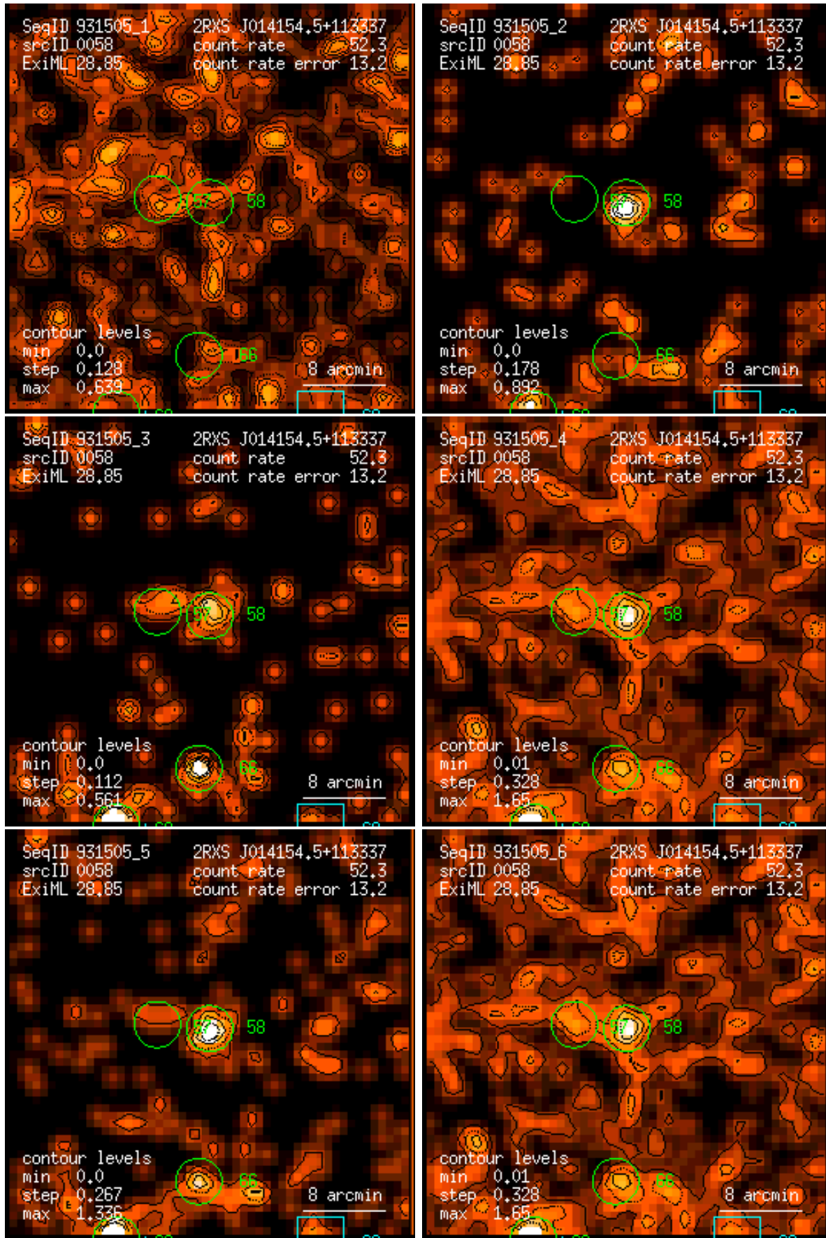
Figure 58: RASS 931505: detection 0058: band rate images, Gaussian filter: (1) PSPC channels 11 – 41, (2) 52 – 90, (3) 91 – 201, (4) 11 – 235, (5) 52 – 201, (6) 11 – 201. Broad band rates in counts/ks. Band rate contour levels in counts/ks/arcmin 2 .
