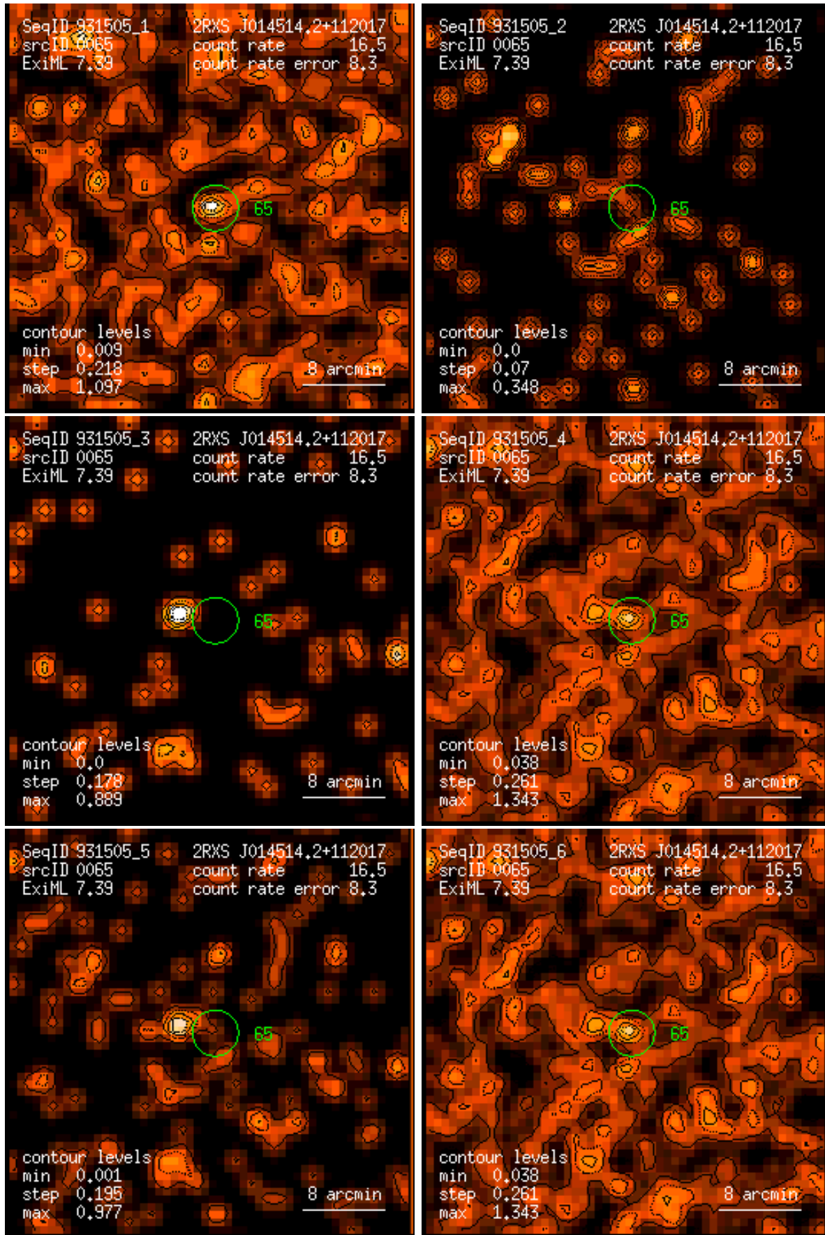
Figure 65: RASS 931505: detection 0065: band rate images, Gaussian filter: (1) PSPC channels 11 – 41, (2) 52 – 90, (3) 91 – 201, (4) 11 – 235, (5) 52 – 201, (6) 11 – 201. Broad band rates in counts/ks. Band rate contour levels in counts/ks/arcmin 2 .
