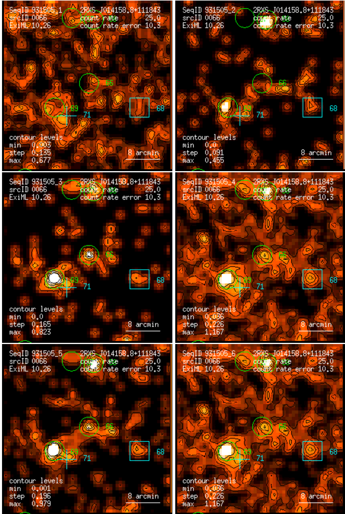
Figure 66: RASS 931505: detection 0066: band rate images, Gaussian filter: (1) PSPC channels 11 – 41, (2) 52 – 90, (3) 91 – 201, (4) 11 – 235, (5) 52 – 201, (6) 11 – 201. Broad band rates in counts/ks. Band rate contour levels in counts/ks/arcmin 2 .
