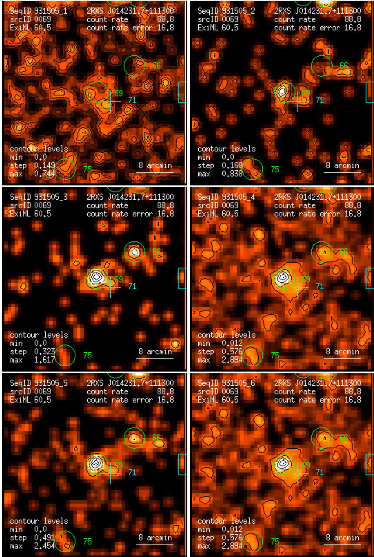
Figure 69: RASS 931505: detection 0069: band rate images, Gaussian filter: (1) PSPC channels 11 – 41, (2) 52 – 90, (3) 91 – 201, (4) 11 – 235, (5) 52 – 201, (6) 11 – 201. Broad band rates in counts/ks. Band rate contour levels in counts/ks/arcmin 2 .
