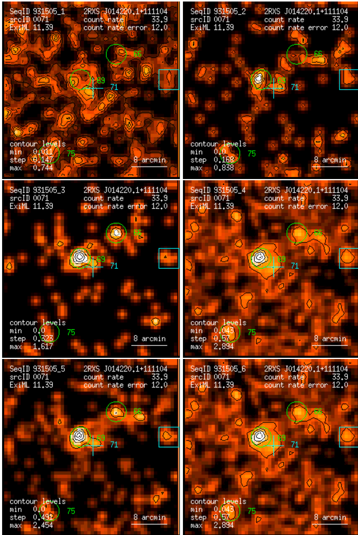
Figure 71: RASS 931505: detection 0071: band rate images, Gaussian filter: (1) PSPC channels 11 – 41, (2) 52 – 90, (3) 91 – 201, (4) 11 – 235, (5) 52 – 201, (6) 11 – 201. Broad band rates in counts/ks. Band rate contour levels in counts/ks/arcmin 2 .
