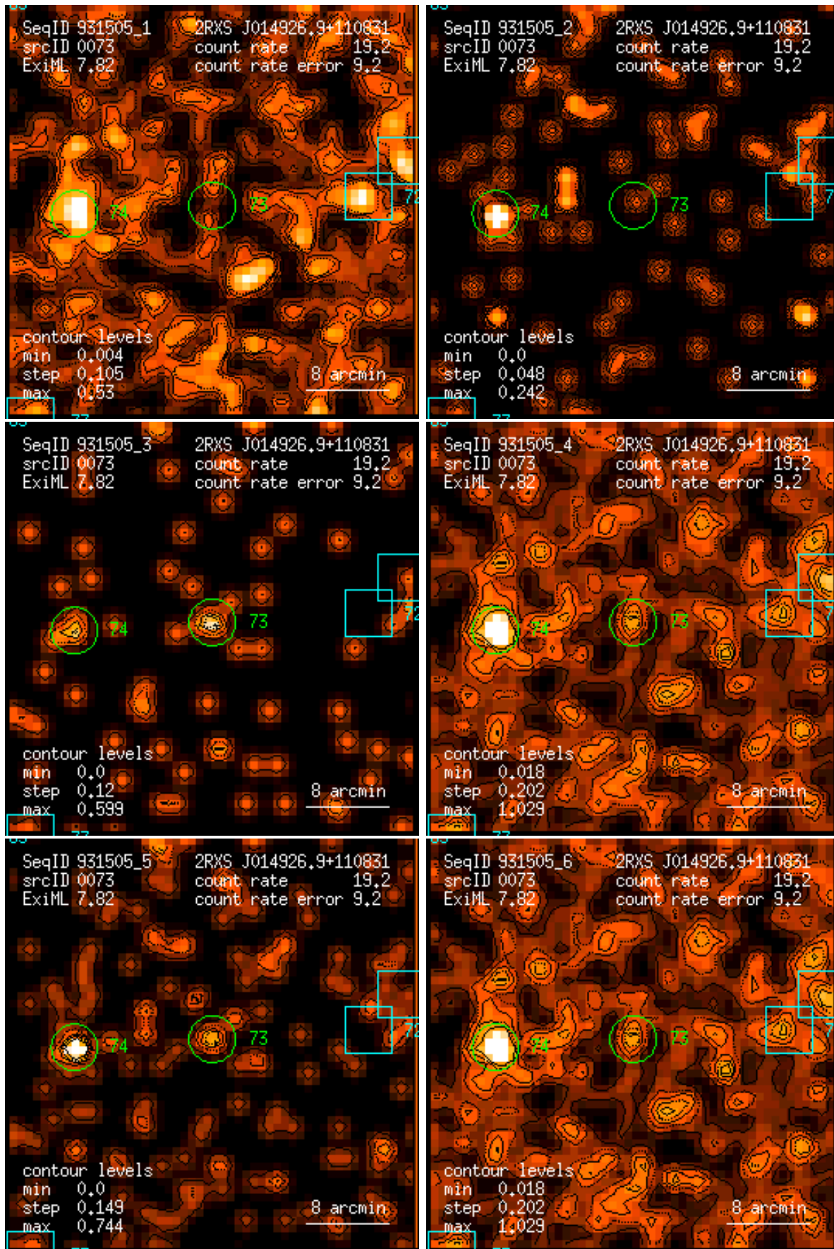
Figure 73: RASS 931505: detection 0073: band rate images, Gaussian filter: (1) PSPC channels 11 – 41, (2) 52 – 90, (3) 91 – 201, (4) 11 – 235, (5) 52 – 201, (6) 11 – 201. Broad band rates in counts/ks. Band rate contour levels in counts/ks/arcmin 2 .
