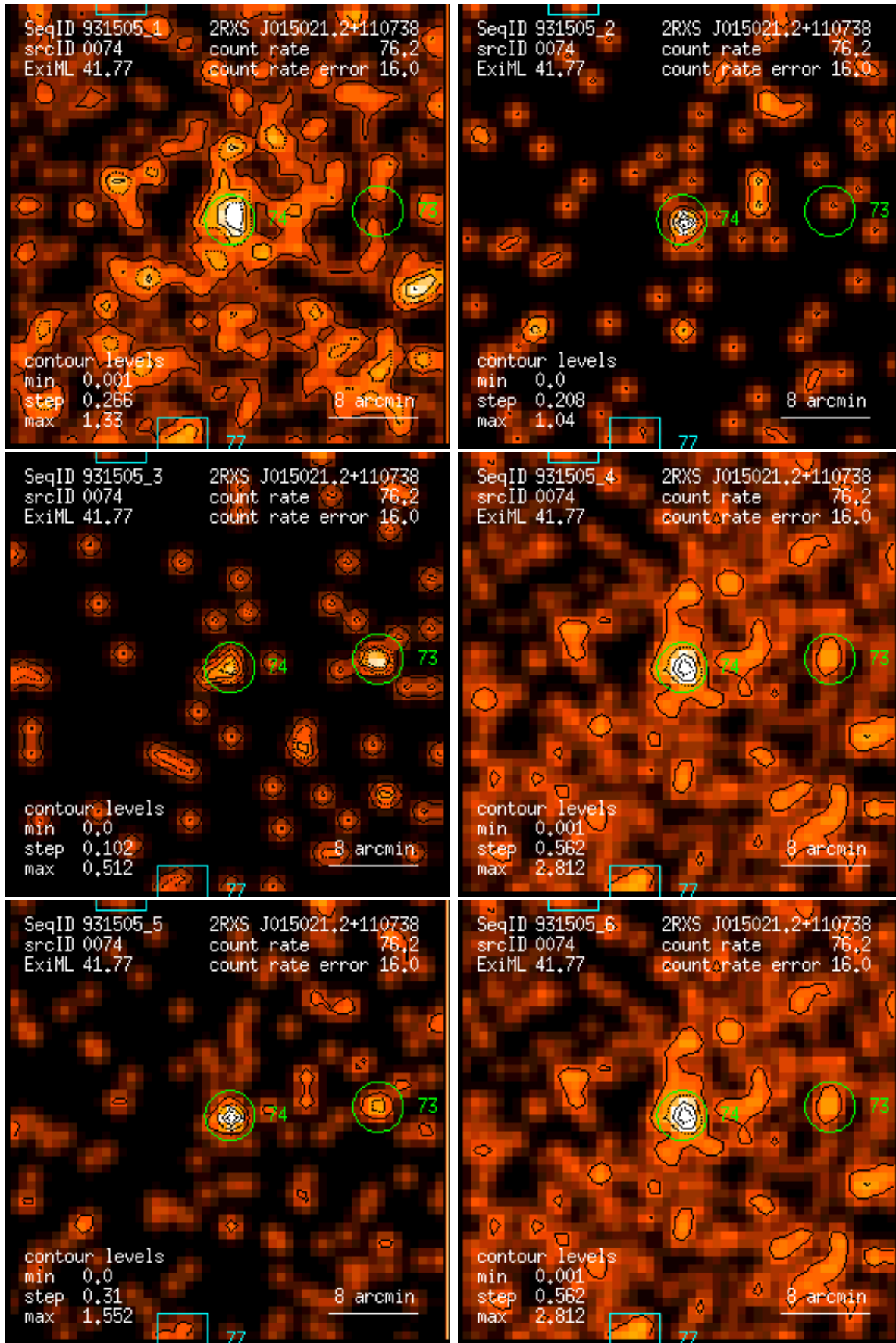
Figure 74: RASS 931505: detection 0074: band rate images, Gaussian filter: (1) PSPC channels 11 – 41, (2) 52 – 90, (3) 91 – 201, (4) 11 – 235, (5) 52 – 201, (6) 11 – 201. Broad band rates in counts/ks. Band rate contour levels in counts/ks/arcmin 2 .
