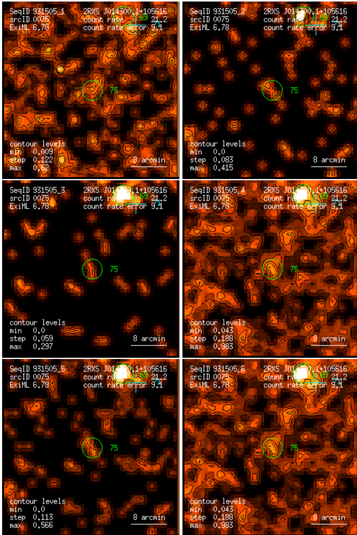
Figure 75: RASS 931505: detection 0075: band rate images, Gaussian filter: (1) PSPC channels 11 – 41, (2) 52 – 90, (3) 91 – 201, (4) 11 – 235, (5) 52 – 201, (6) 11 – 201. Broad band rates in counts/ks. Band rate contour levels in counts/ks/arcmin 2 .
