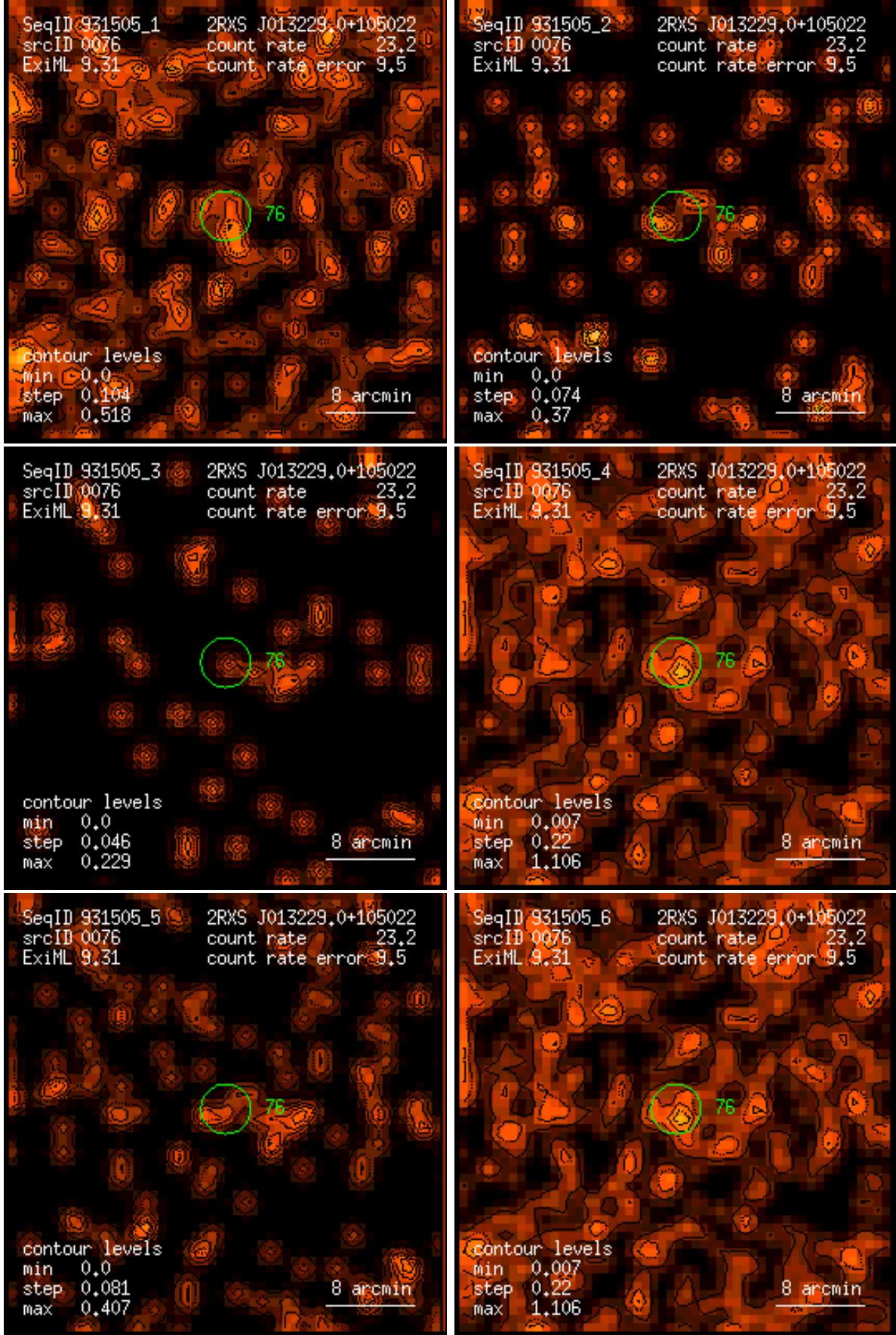
Figure 76: RASS 931505: detection 0076: band rate images, Gaussian filter: (1) PSPC channels 11 – 41, (2) 52 – 90, (3) 91 – 201, (4) 11 – 235, (5) 52 – 201, (6) 11 – 201. Broad band rates in counts/ks. Band rate contour levels in counts/ks/arcmin 2 .
