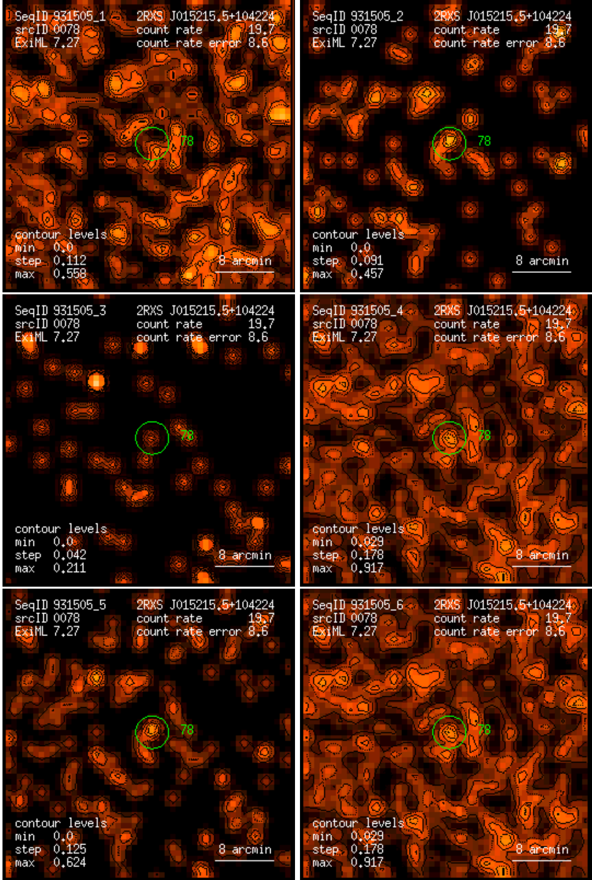
Figure 78: RASS 931505: detection 0078: band rate images, Gaussian filter: (1) PSPC channels 11 – 41, (2) 52 – 90, (3) 91 – 201, (4) 11 – 235, (5) 52 – 201, (6) 11 – 201. Broad band rates in counts/ks. Band rate contour levels in counts/ks/arcmin 2 .
