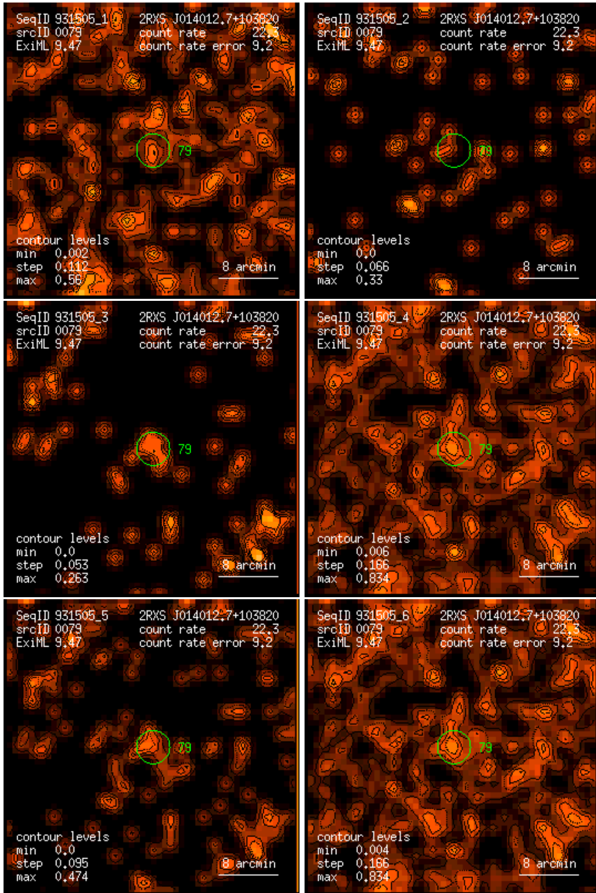
Figure 79: RASS 931505: detection 0079: band rate images, Gaussian filter: (1) PSPC channels 11 – 41, (2) 52 – 90, (3) 91 – 201, (4) 11 – 235, (5) 52 – 201, (6) 11 – 201. Broad band rates in counts/ks. Band rate contour levels in counts/ks/arcmin 2 .
