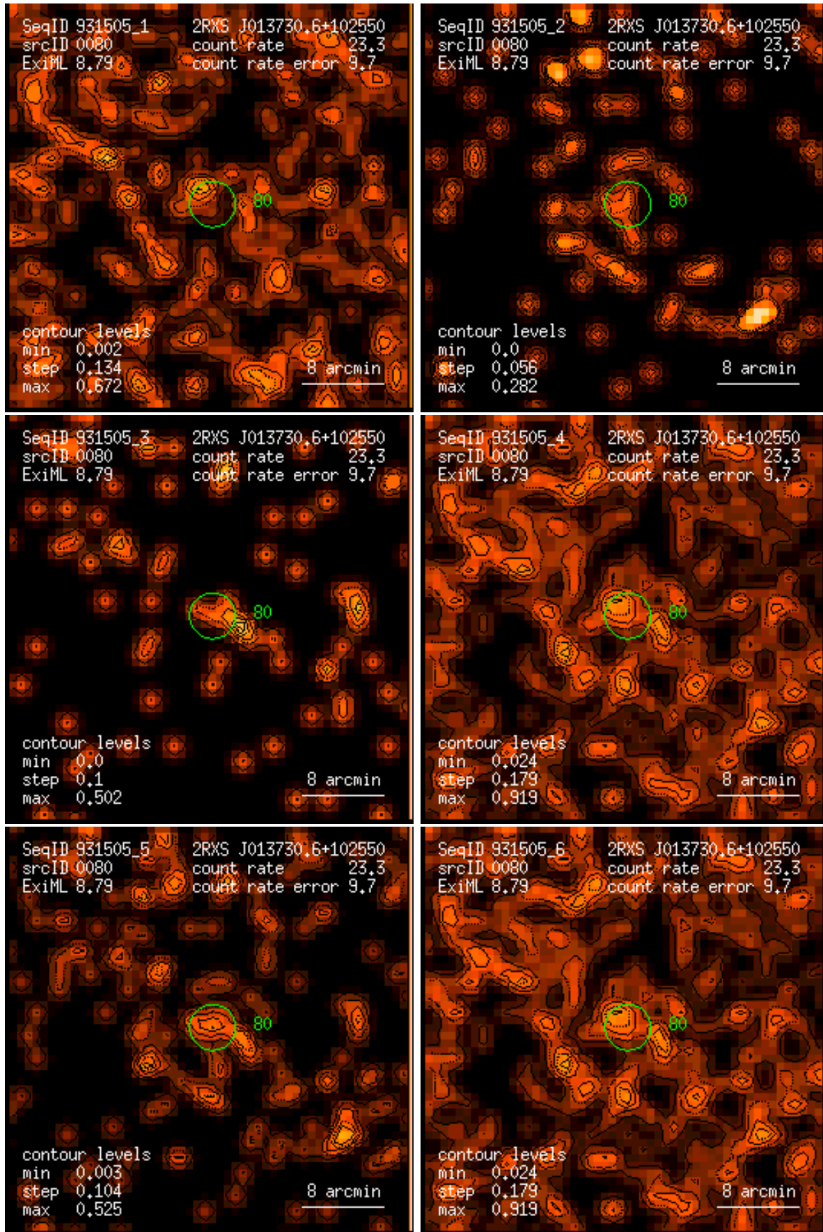
Figure 80: RASS 931505: detection 0080: band rate images, Gaussian filter: (1) PSPC channels 11 – 41, (2) 52 – 90, (3) 91 – 201, (4) 11 – 235, (5) 52 – 201, (6) 11 – 201. Broad band rates in counts/ks. Band rate contour levels in counts/ks/arcmin 2 .
