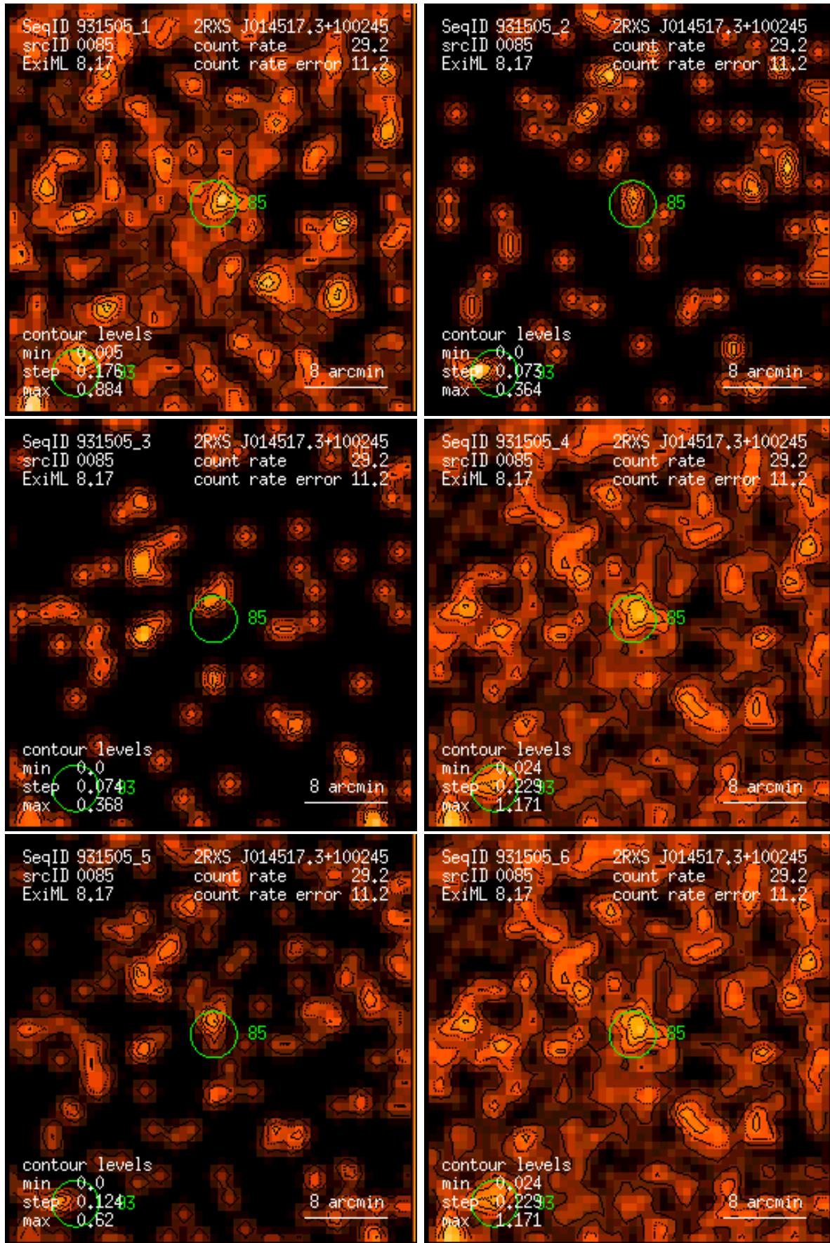
Figure 85: RASS 931505: detection 0085: band rate images, Gaussian filter: (1) PSPC channels 11 – 41, (2) 52 – 90, (3) 91 – 201, (4) 11 – 235, (5) 52 – 201, (6) 11 – 201. Broad band rates in counts/ks. Band rate contour levels in counts/ks/arcmin 2 .
