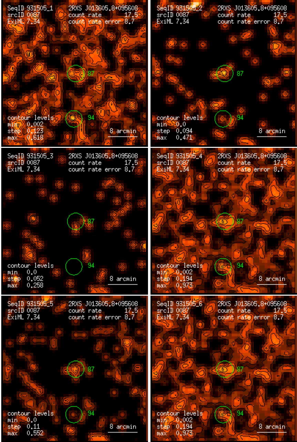
Figure 87: RASS 931505: detection 0087: band rate images, Gaussian filter: (1) PSPC channels 11 – 41, (2) 52 – 90, (3) 91 – 201, (4) 11 – 235, (5) 52 – 201, (6) 11 – 201. Broad band rates in counts/ks. Band rate contour levels in counts/ks/arcmin 2 .
