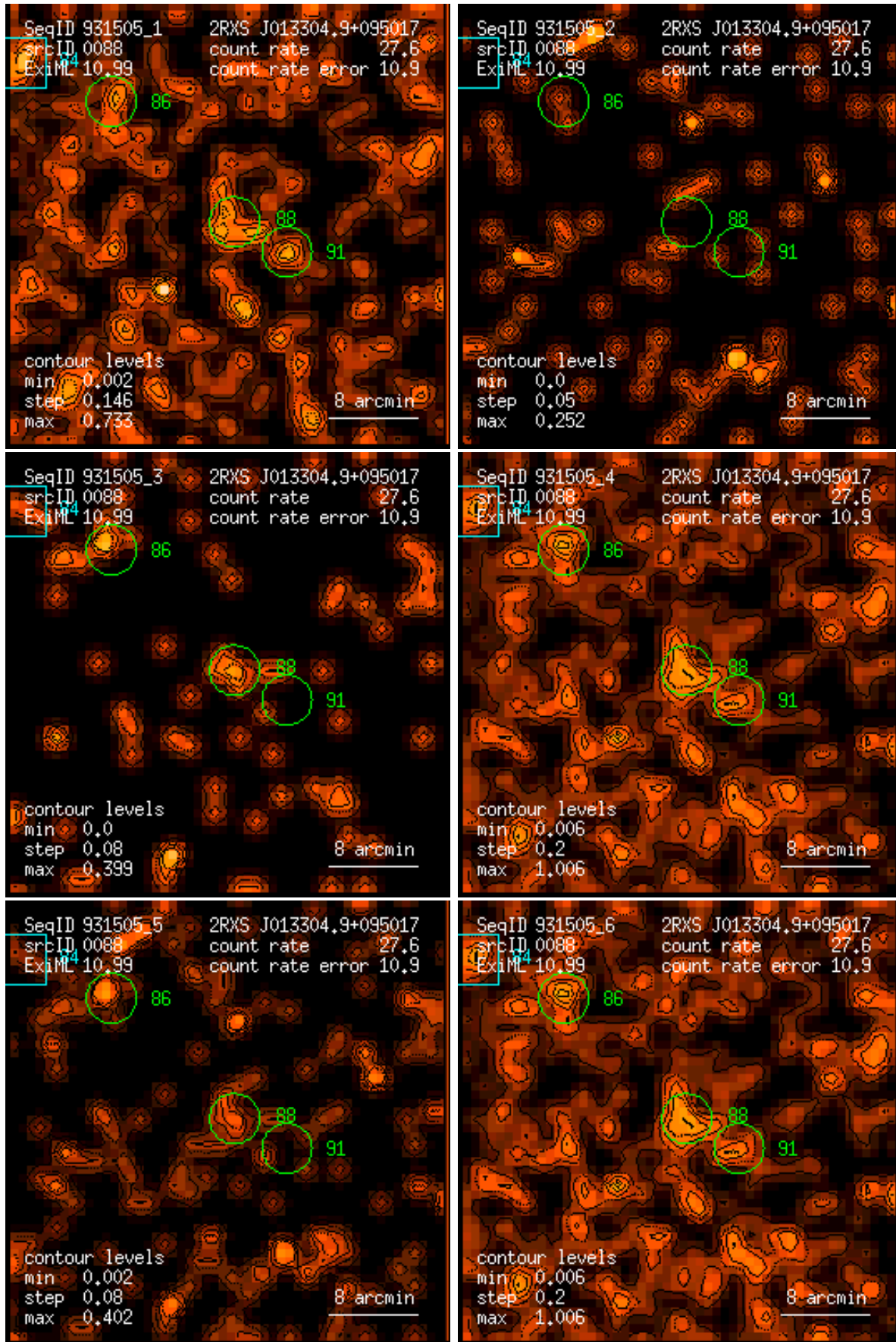
Figure 88: RASS 931505: detection 0088: band rate images, Gaussian filter: (1) PSPC channels 11 – 41, (2) 52 – 90, (3) 91 – 201, (4) 11 – 235, (5) 52 – 201, (6) 11 – 201. Broad band rates in counts/ks. Band rate contour levels in counts/ks/arcmin 2 .
