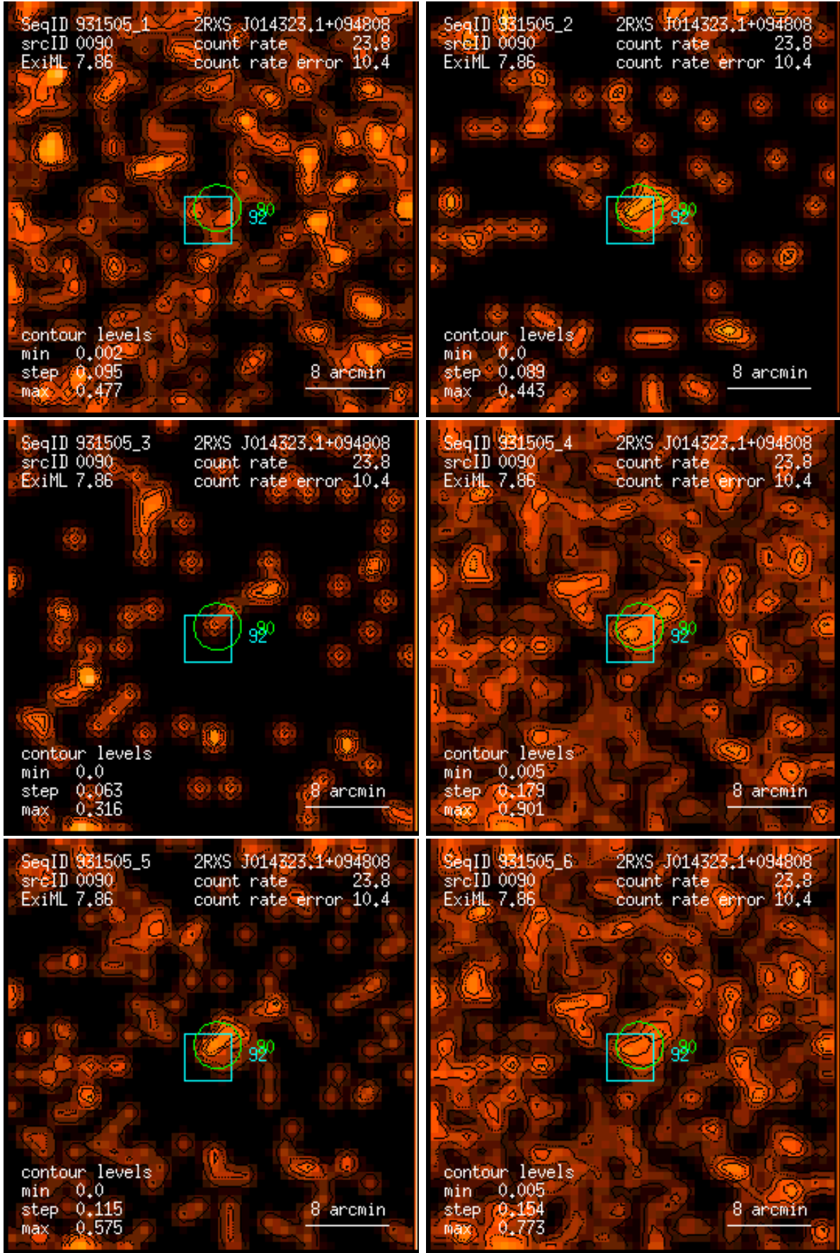
Figure 90: RASS 931505: detection 0090: band rate images, Gaussian filter: (1) PSPC channels 11 – 41, (2) 52 – 90, (3) 91 – 201, (4) 11 – 235, (5) 52 – 201, (6) 11 – 201. Broad band rates in counts/ks. Band rate contour levels in counts/ks/arcmin 2 .
