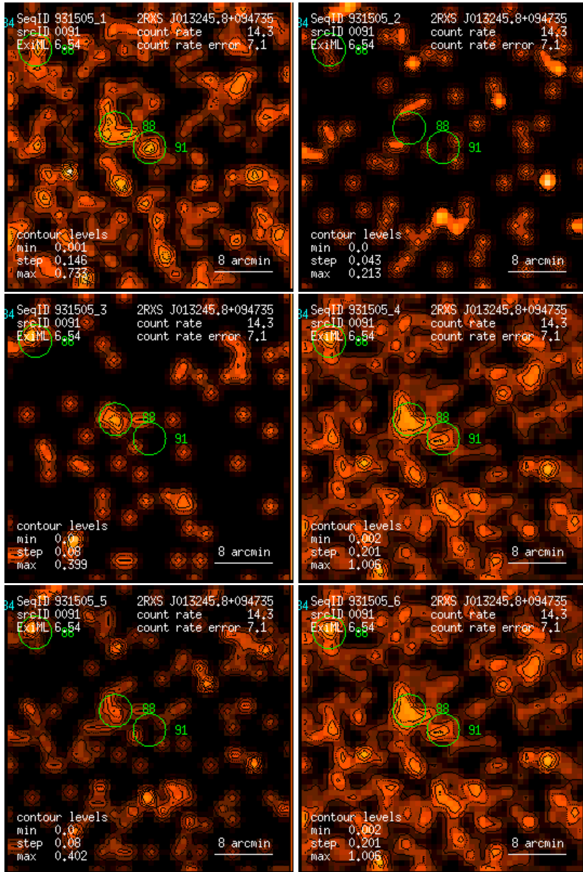
Figure 91: RASS 931505: detection 0091: band rate images, Gaussian filter: (1) PSPC channels 11 – 41, (2) 52 – 90, (3) 91 – 201, (4) 11 – 235, (5) 52 – 201, (6) 11 – 201. Broad band rates in counts/ks. Band rate contour levels in counts/ks/arcmin 2 .
