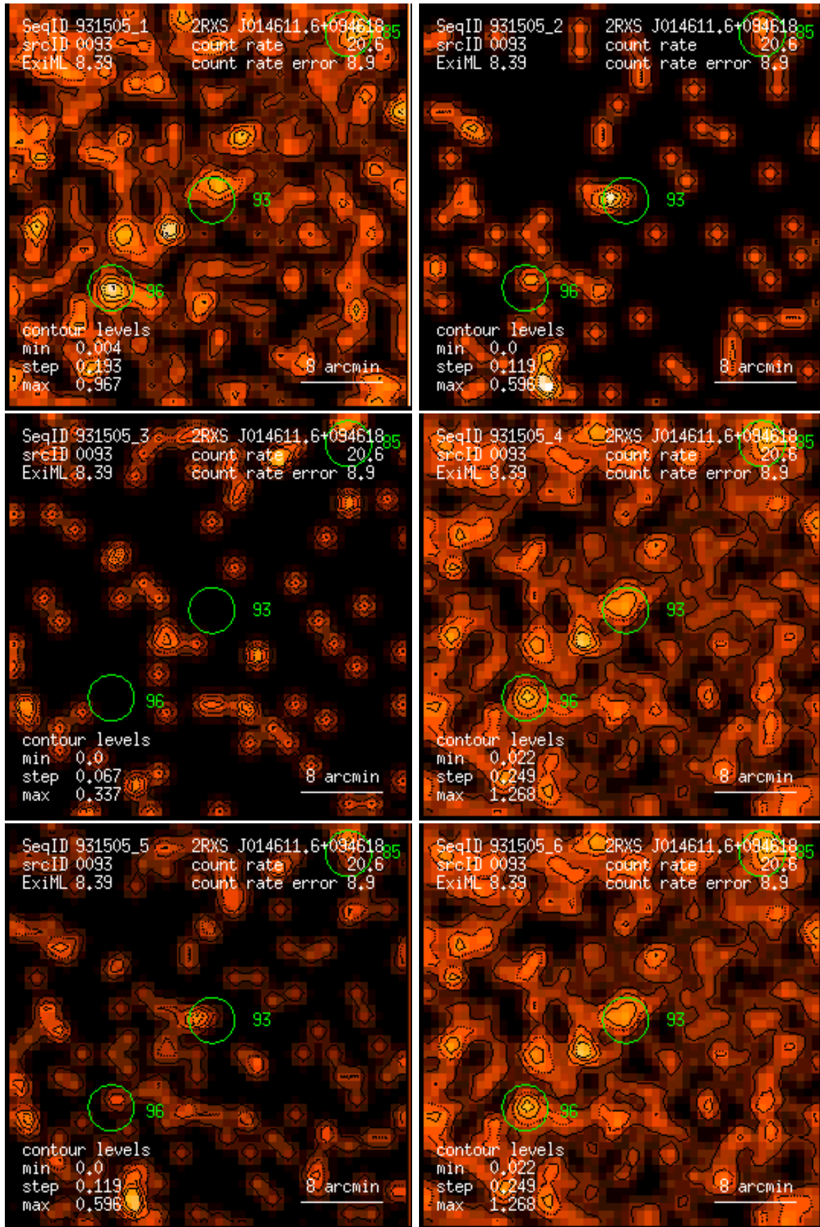
Figure 93: RASS 931505: detection 0093: band rate images, Gaussian filter: (1) PSPC channels 11 – 41, (2) 52 – 90, (3) 91 – 201, (4) 11 – 235, (5) 52 – 201, (6) 11 – 201. Broad band rates in counts/ks. Band rate contour levels in counts/ks/arcmin 2 .
