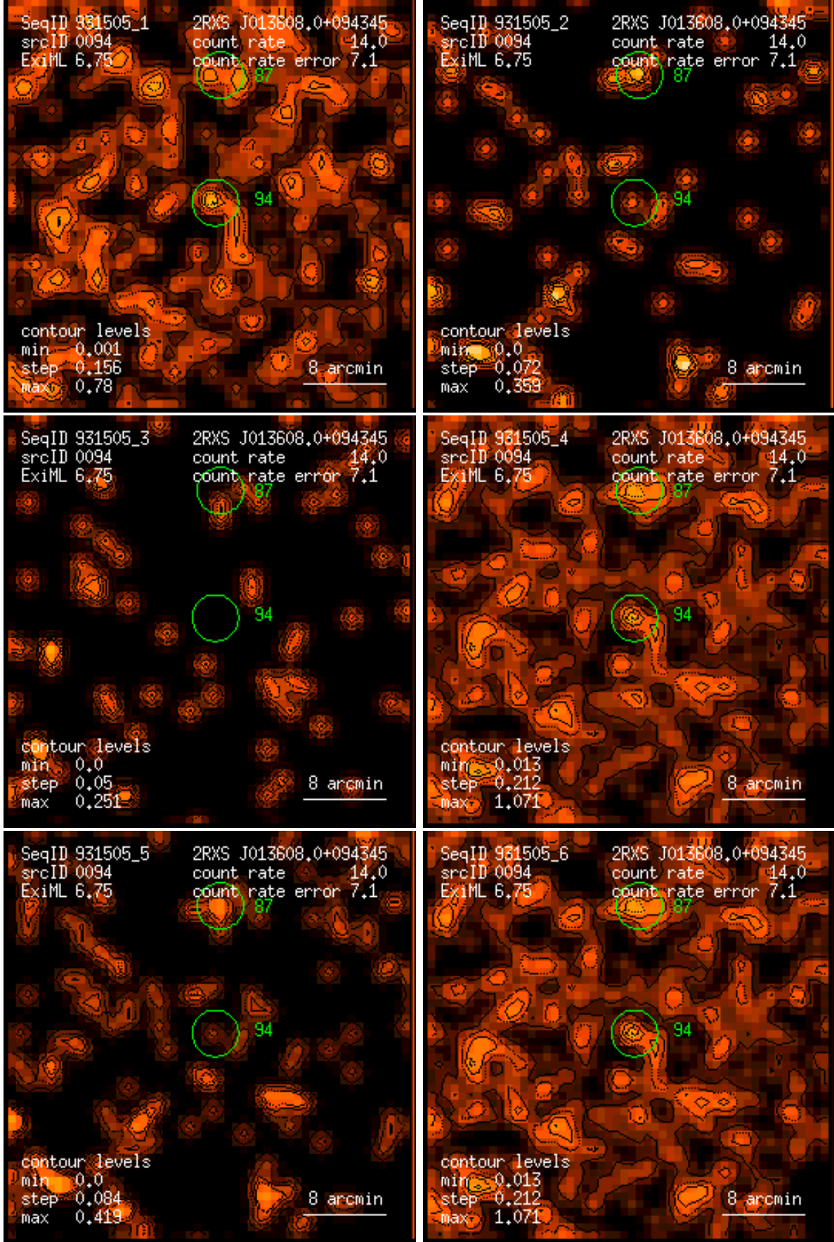
Figure 94: RASS 931505: detection 0094: band rate images, Gaussian filter: (1) PSPC channels 11 – 41, (2) 52 – 90, (3) 91 – 201, (4) 11 – 235, (5) 52 – 201, (6) 11 – 201. Broad band rates in counts/ks. Band rate contour levels in counts/ks/arcmin 2 .
