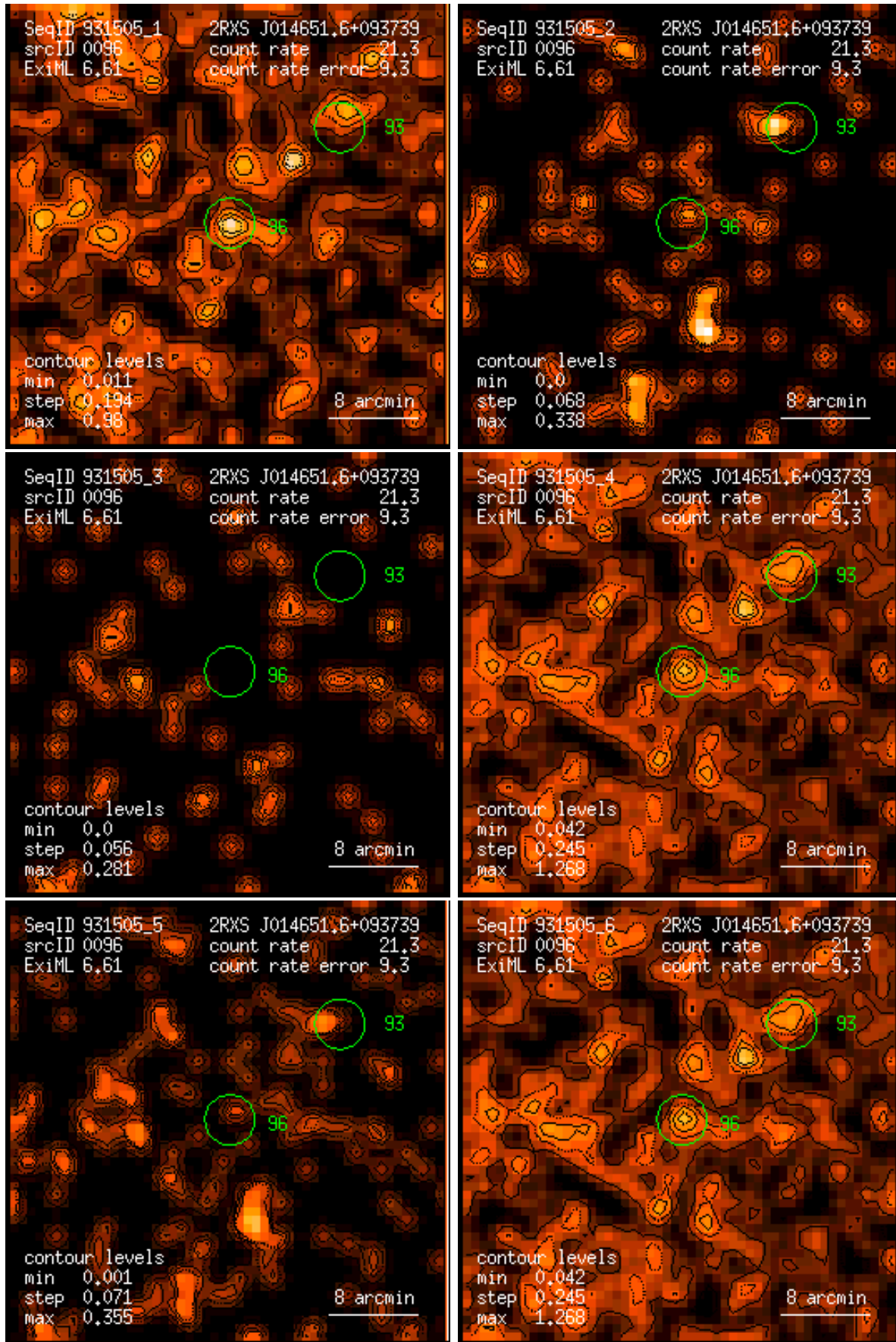
Figure 96: RASS 931505: detection 0096: band rate images, Gaussian filter: (1) PSPC channels 11 – 41, (2) 52 – 90, (3) 91 – 201, (4) 11 – 235, (5) 52 – 201, (6) 11 – 201. Broad band rates in counts/ks. Band rate contour levels in counts/ks/arcmin 2 .
