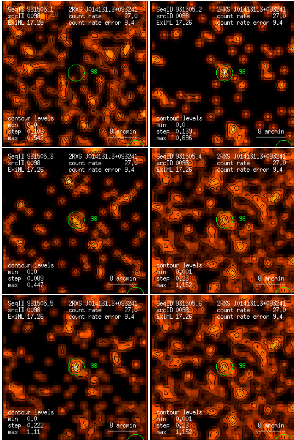
Figure 98: RASS 931505: detection 0098: band rate images, Gaussian filter: (1) PSPC channels 11 – 41, (2) 52 – 90, (3) 91 – 201, (4) 11 – 235, (5) 52 – 201, (6) 11 – 201. Broad band rates in counts/ks. Band rate contour levels in counts/ks/arcmin 2 .
