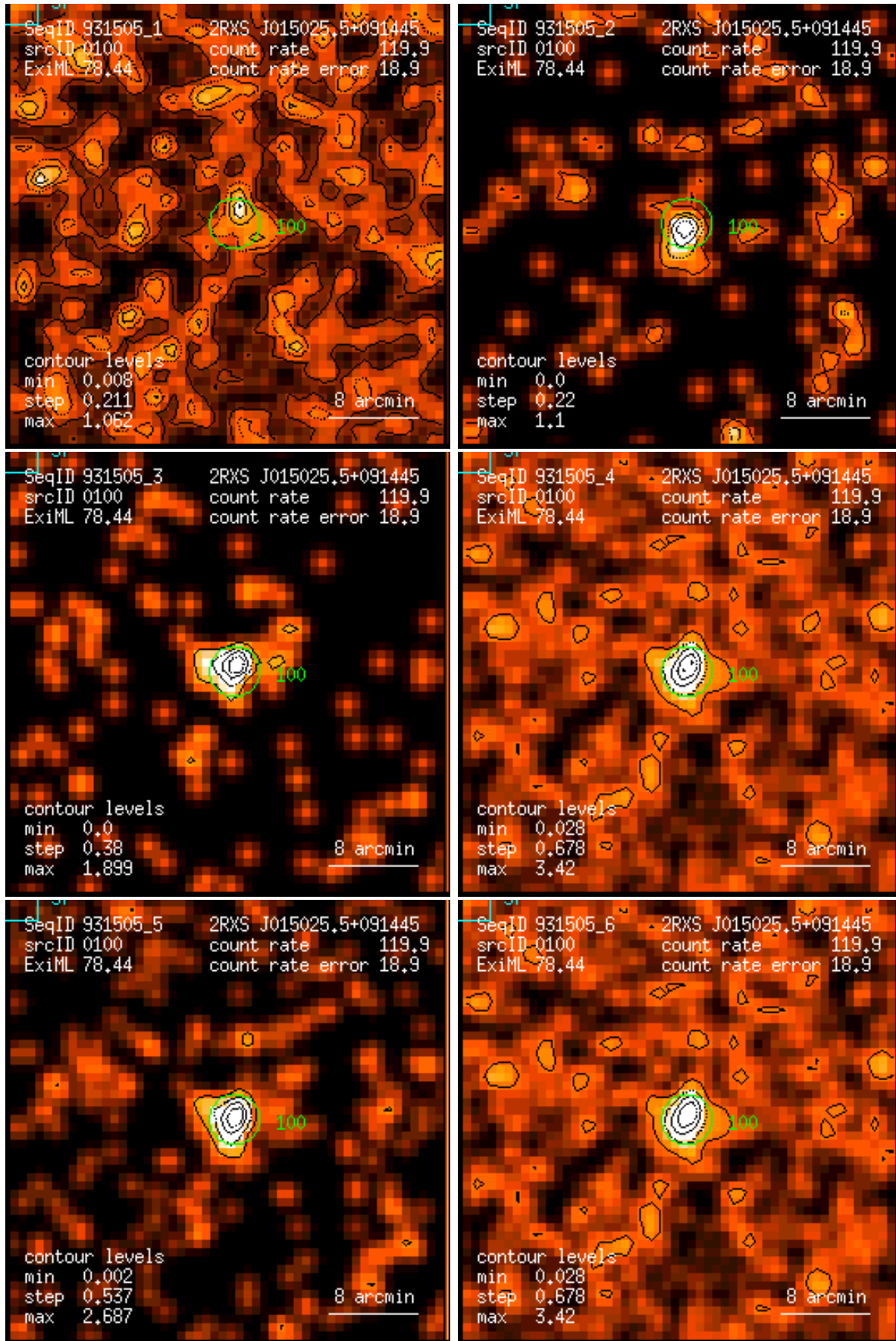
Figure 100: RASS 931505: detection 0100: band rate images, Gaussian filter: (1) PSPC channels 11 – 41, (2) 52 – 90, (3) 91 – 201, (4) 11 – 235, (5) 52 – 201, (6) 11 – 201. Broad band rates in counts/ks. Band rate contour levels in counts/ks/arcmin 2 .
