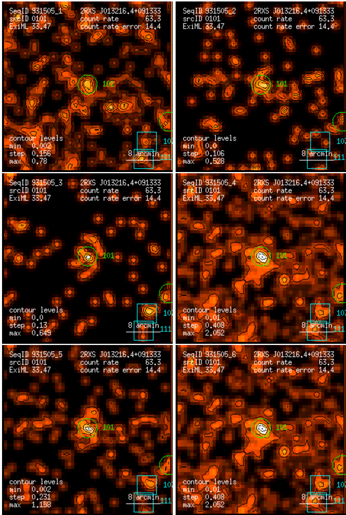
Figure 101: RASS 931505: detection 0101: band rate images, Gaussian filter: (1) PSPC channels 11 – 41, (2) 52 – 90, (3) 91 – 201, (4) 11 – 235, (5) 52 – 201, (6) 11 – 201. Broad band rates in counts/ks. Band rate contour levels in counts/ks/arcmin 2 .
