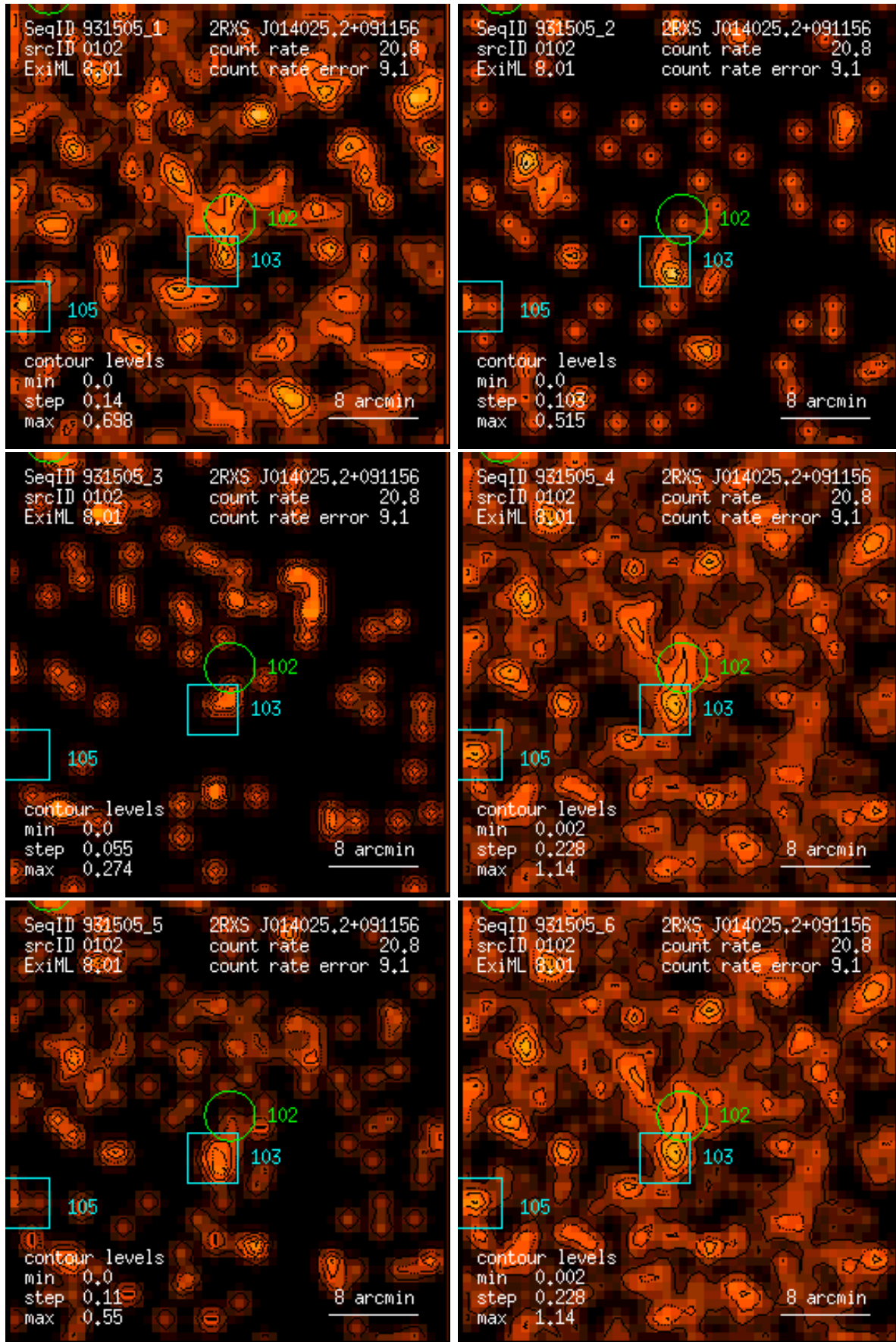
Figure 102: RASS 931505: detection 0102: band rate images, Gaussian filter: (1) PSPC channels 11 – 41, (2) 52 – 90, (3) 91 – 201, (4) 11 – 235, (5) 52 – 201, (6) 11 – 201. Broad band rates in counts/ks. Band rate contour levels in counts/ks/arcmin 2 .
